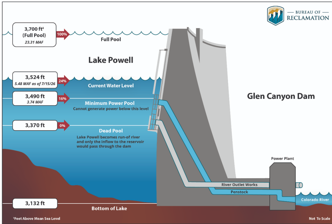
Figure 1-3 Glen Canyon Dam Key Elevations
