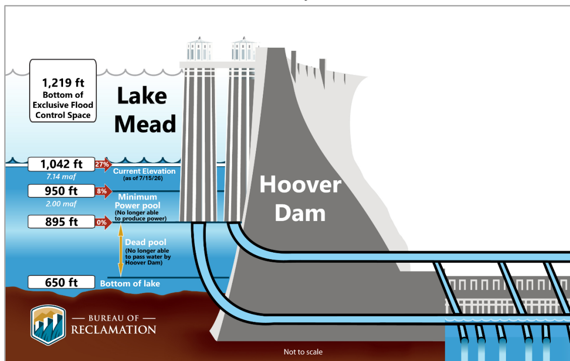
Figure 1-5 Hoover Dam Key Elevations
