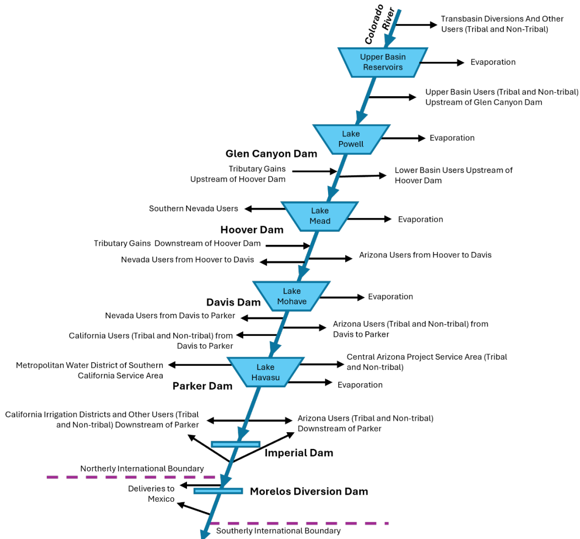
Figure 1-1 Colorado River Reservoirs and Diversions
