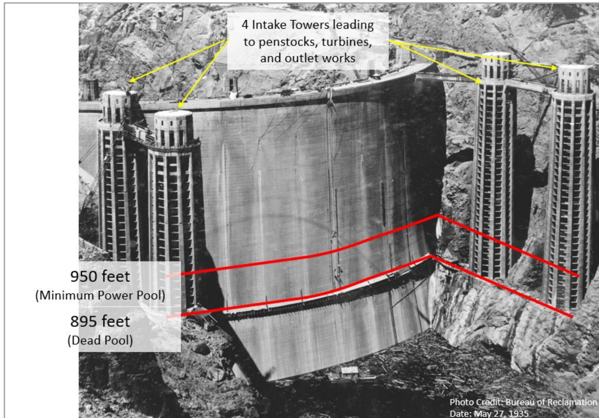
Figure 1-6 Hoover Dam in 1935 (before filling)
