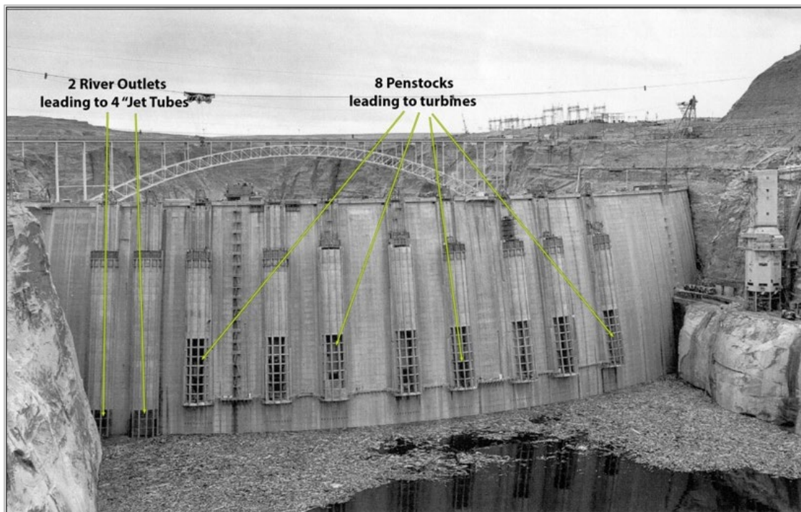
Figure 1-4 Glen Canyon Dam in 1963 (Before Filling)
