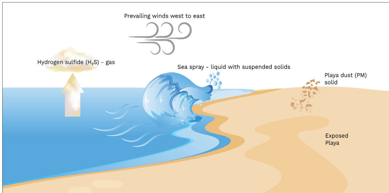
FIGURE 9. Salton Sea Contaminants — Gases, Liquids, and Solids
