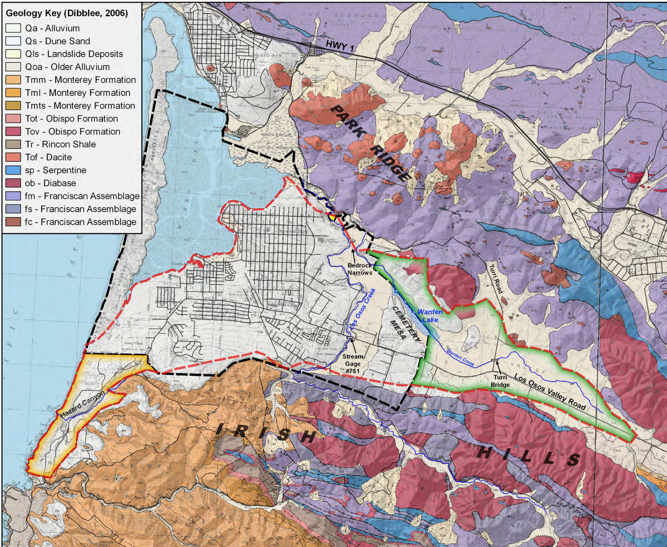
Figure 2 - Basin Geology
