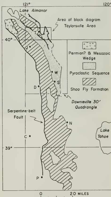
Figure 1. Index map showing the relations of the Taylorsville area to the regional geology. Taylorsville (T), Quincy (Q), Wades Lake (W), Sierra Buttes (S), Downieville (D), North Fork American River where it crosses the top of the Shoo Fly Formation (N), Calfax (C), and Placerville (P) are represented on the map by letters.
