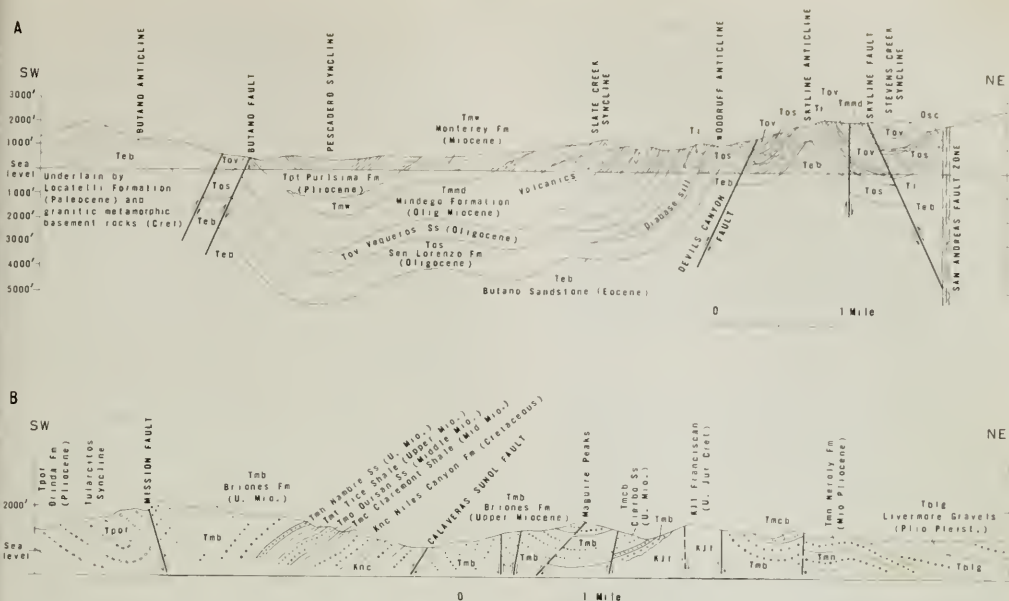
Figure 5. Typical cross sections. Cross section A is modified from Cummings, Touring, and Brabb, 1962 and is in area of column A, figure 4. Cross section B is modified from Hall, 1958, and is in area of column B, figure 4.
