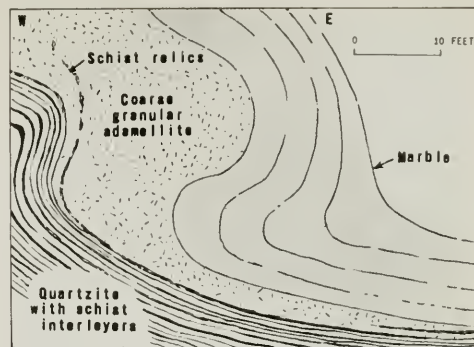
Figure 6. Coarse-grained adamellite intruded between marble and quartzite layers during first folding of Sur series. View is approximately along fold axes. Sketched from exposure on vertical canyon wall, 5\frac{1}{2} miles west-northwest of Junipero Serra Peak.
