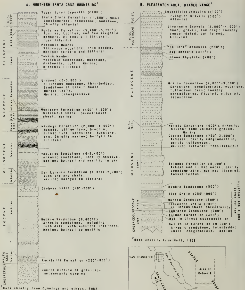
Figure 4. Representative columnar sections of "overlying blanket" of Cenozoic deposits.
