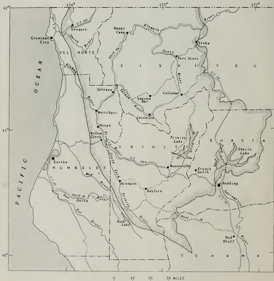
Figure 1. Map of northwestern California showing outline of Klamath Mountains province, major drainage, towns and routes of travel.
