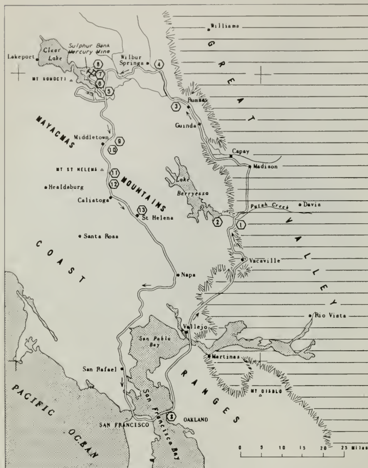
Figure 1. Index map of area between San Francisco and Clear Lake, showing boundary between Coast Ranges and Great Valley and route of field trip. Stops in road log are indicated by numbers in hexagons.
