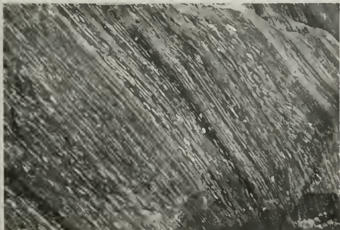
Photo 10. Middle Miocene phosphatic shale facies exposed (A, left) in sea cliffs east of Naples in the Ventura Basin, (field of view, .7 m) and (B, right) in the Los Angeles Basin, at Malaga Cove (field of view, 1.8 m).
