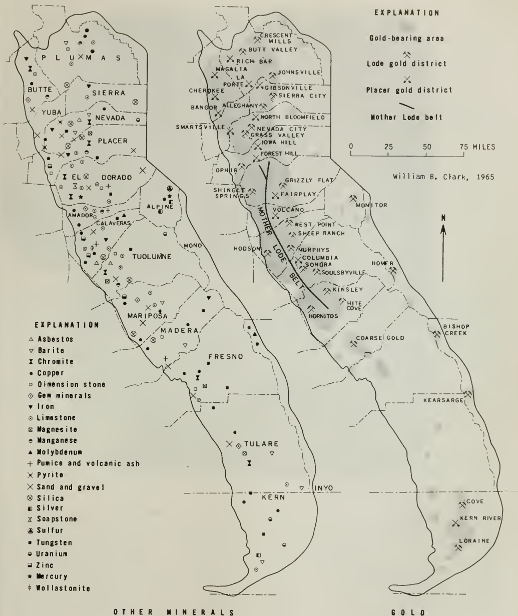
Figure 1. Location of economic deposits of the Sierra Nevada province.
