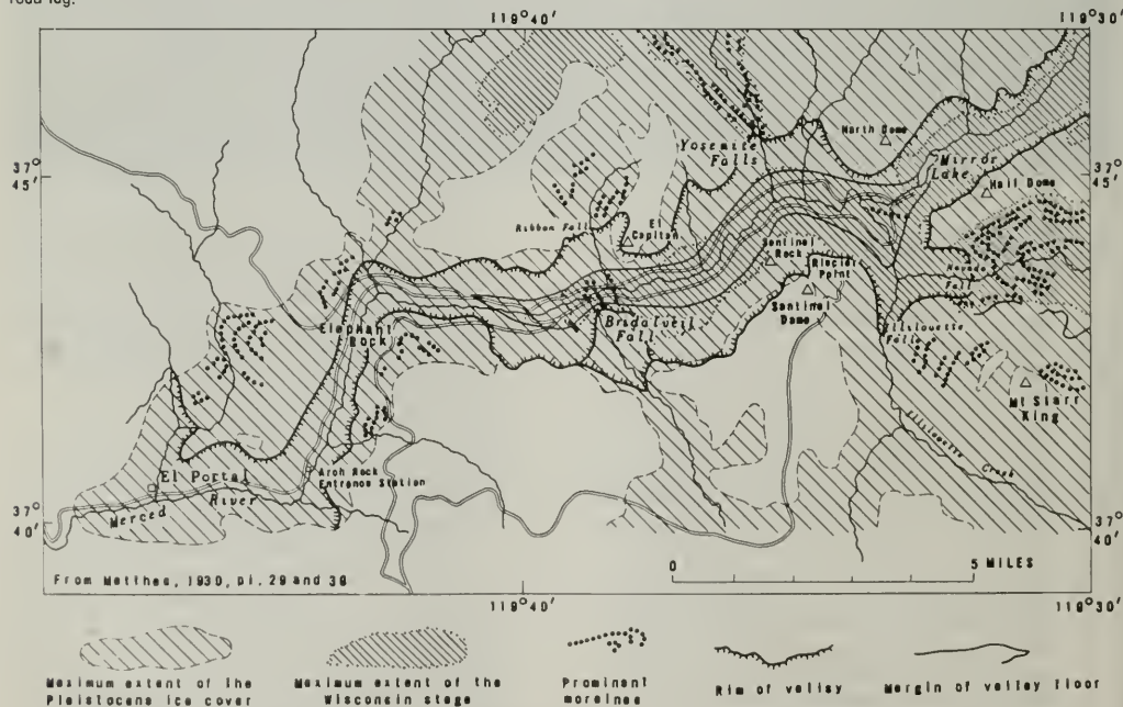
Figure 6. Sketch map showing former extent of glacial ice in and around Yosemite Valley.
