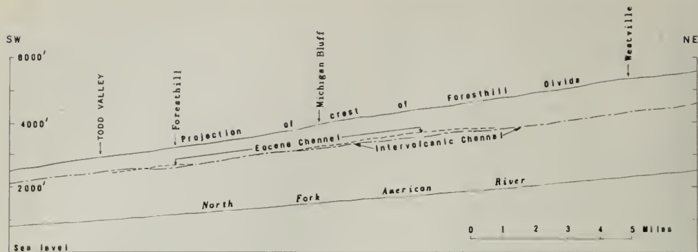
Figure 12. Projection of prevolcanic (Eocene?) and intervalvanic (Pliocene) channels of Forest Hill Divide, and of the North Fork of the American River, onto a vertical plane striking N. 50° E. Data from Ross E. Browne, 1890. For location of projection plane see figure 10. Vertical exaggeration about 10 X.
