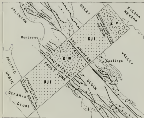
Figure 6. Major structural boundaries of the Coast Ranges, shown by a part of figure 1 redrawn with younger rocks "peeled" from transverse rectangular area to reveal underlying rocks and principal contacts.
