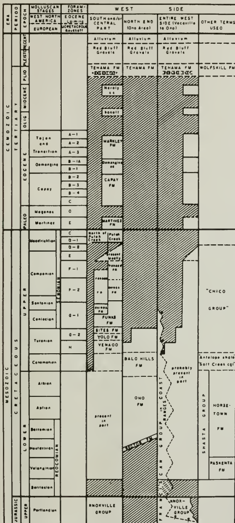
Figure 2. Stratigraphic chart showing units exposed along the west side of the Sacramento Valley. From Lachenbruch (1962).
