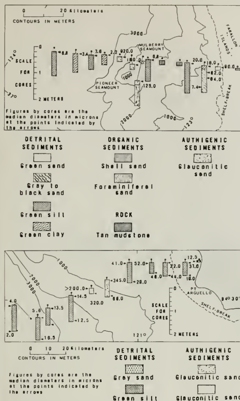
Figure 6. Lithology of surficial deposits off San Francisco (top) and Point Arguello (bottom) as described from cores by Uchupi and Emery (1963).
