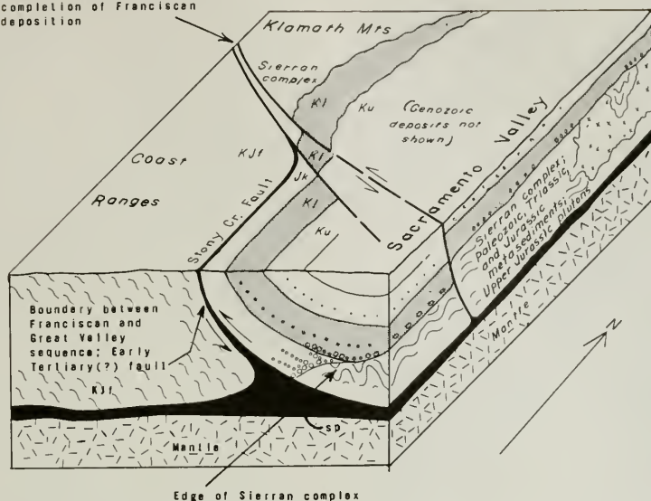
Figure 7. Block diagram showing tentative schematic interpretation of the structural relations in an area west of Red Bluff.
