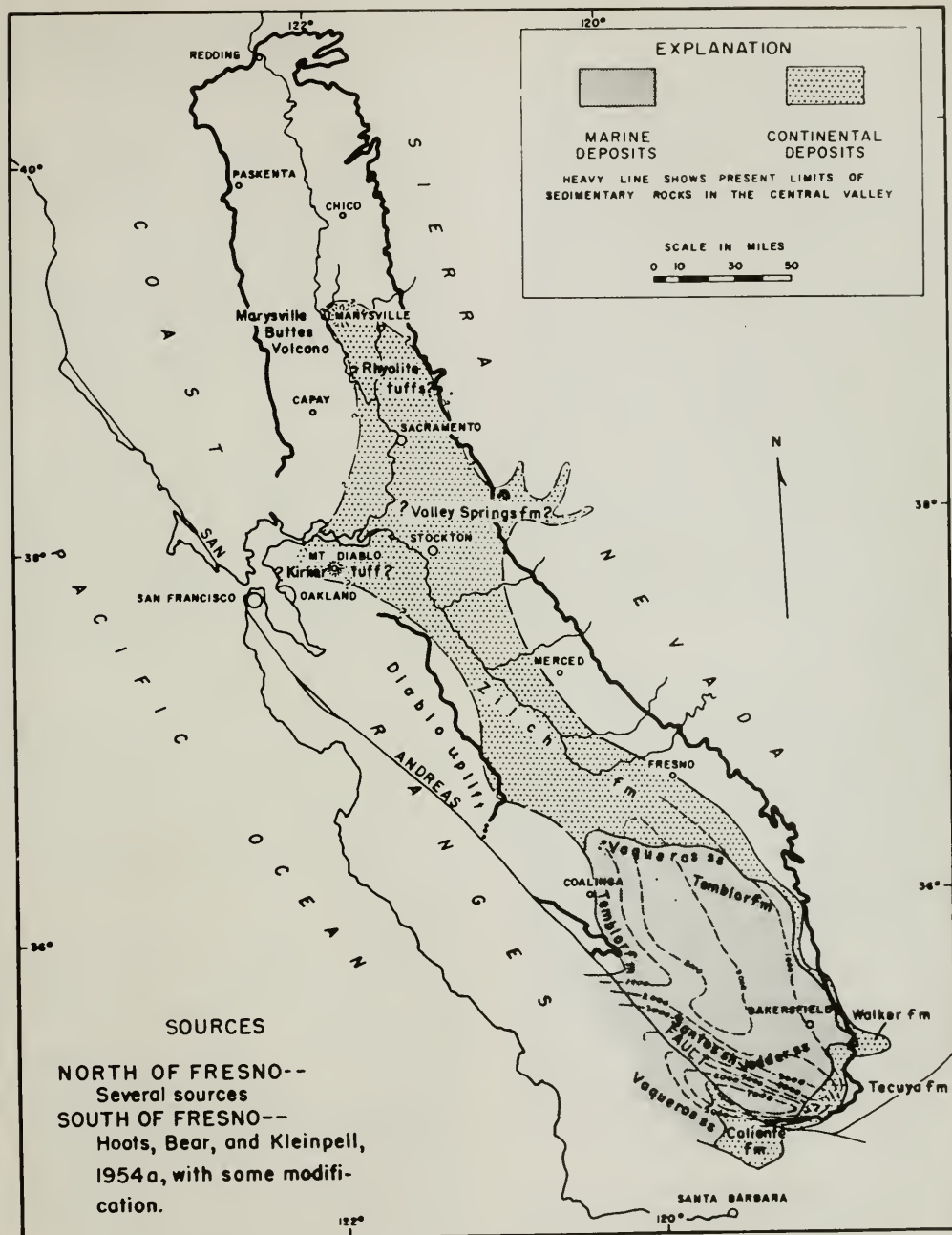
Figure 6. Distribution and thickness of lower Miocene sediments in the Great Valley of the beginning of middle Miocene time. After Reppening (1960, fig. 8).
