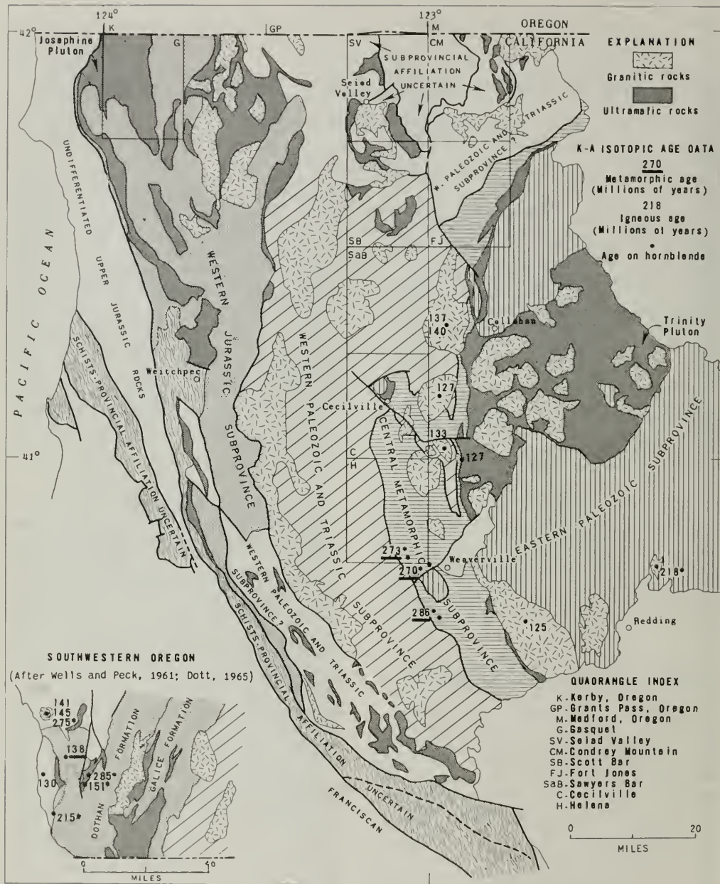
Figure 1. Geologic index map of the Klamath province, northwestern California, showing available isotopic age data, with inset map of southwestern Oregon showing additional isotopic ages. Index map modified after Weed (1963) and Redding (1962) sheets, Geologic Map of California.
