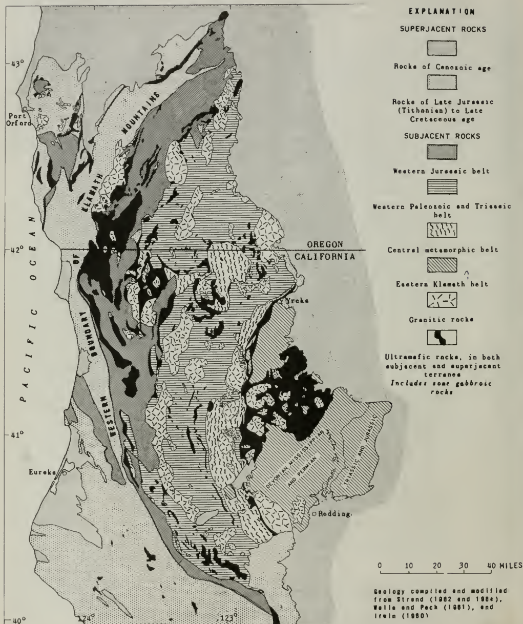
Figure 2. Geologic map of northwestern California and southwestern Oregon.
