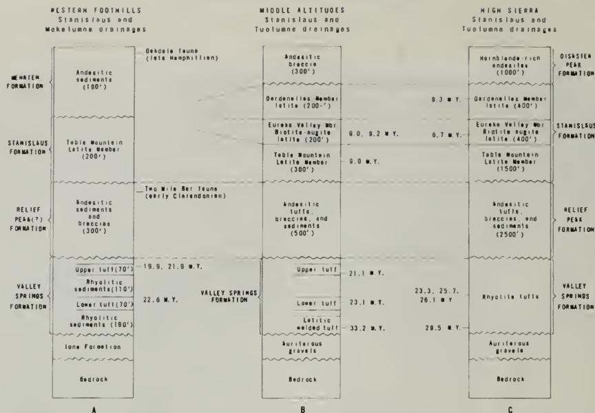
Figure 1. Correlation and summary diagram of Tertiary rocks of the central Sierra Nevada (after Dalrymple, 1964): A, Composite section from Valley Springs Formation type section and Knights Ferry area; B, Composite section from Panderosa Way, Rattlesnake Hill, McKay, and Jawbone Ridge; C, Composite section from Sonora Pass and Rancheria Mountain.
