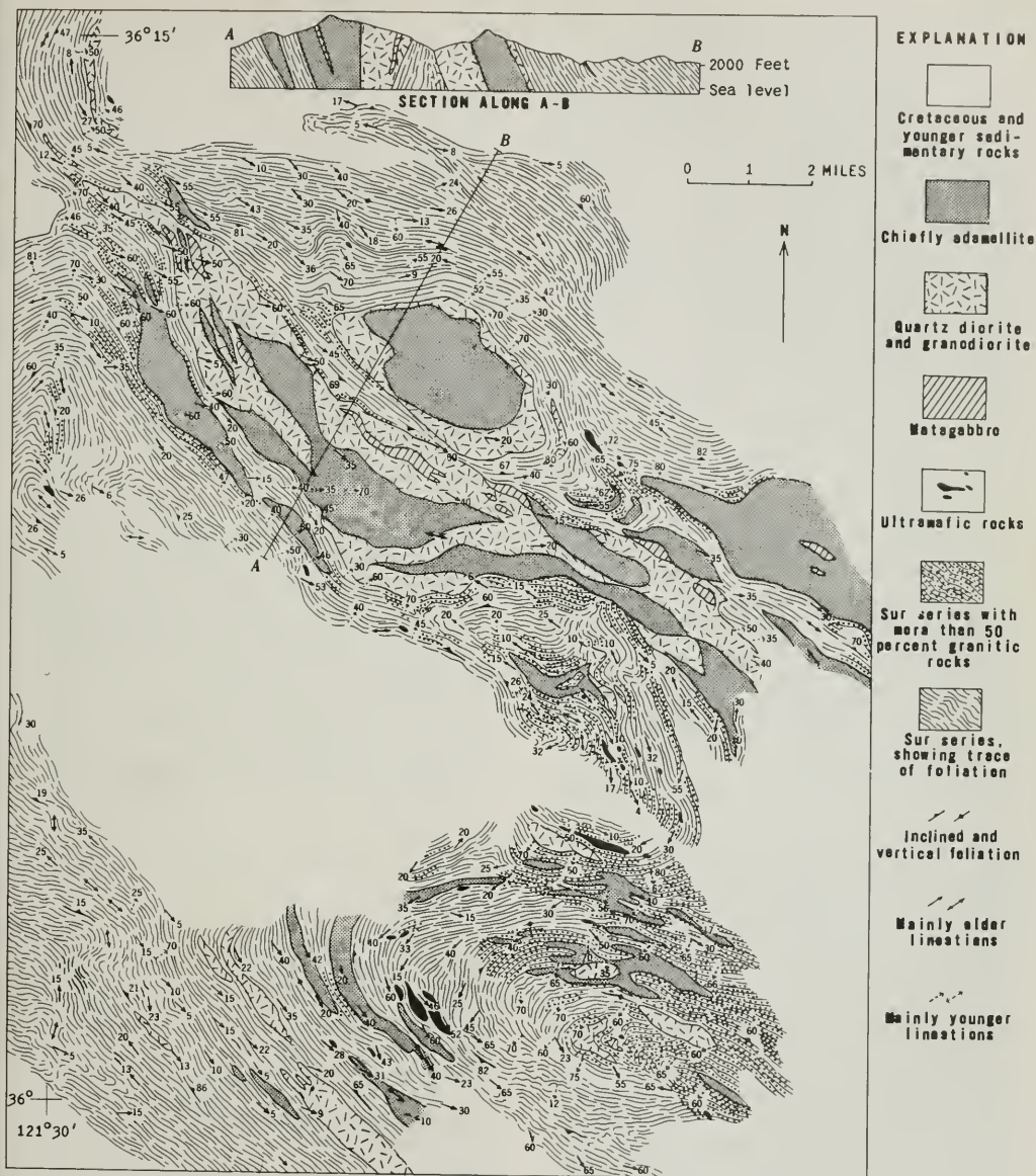
Figure 4. Basement rocks and structures of the Junipero Serrero 15' quadrangle and surroundings. The main figure is a horizontal section at 2,000 feet altitude.
