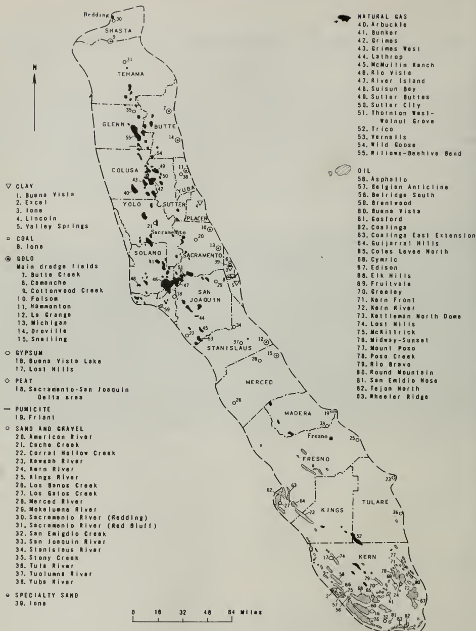
Figure 1. Map of the Great Valley, showing the location of the principal economic mineral deposits.
