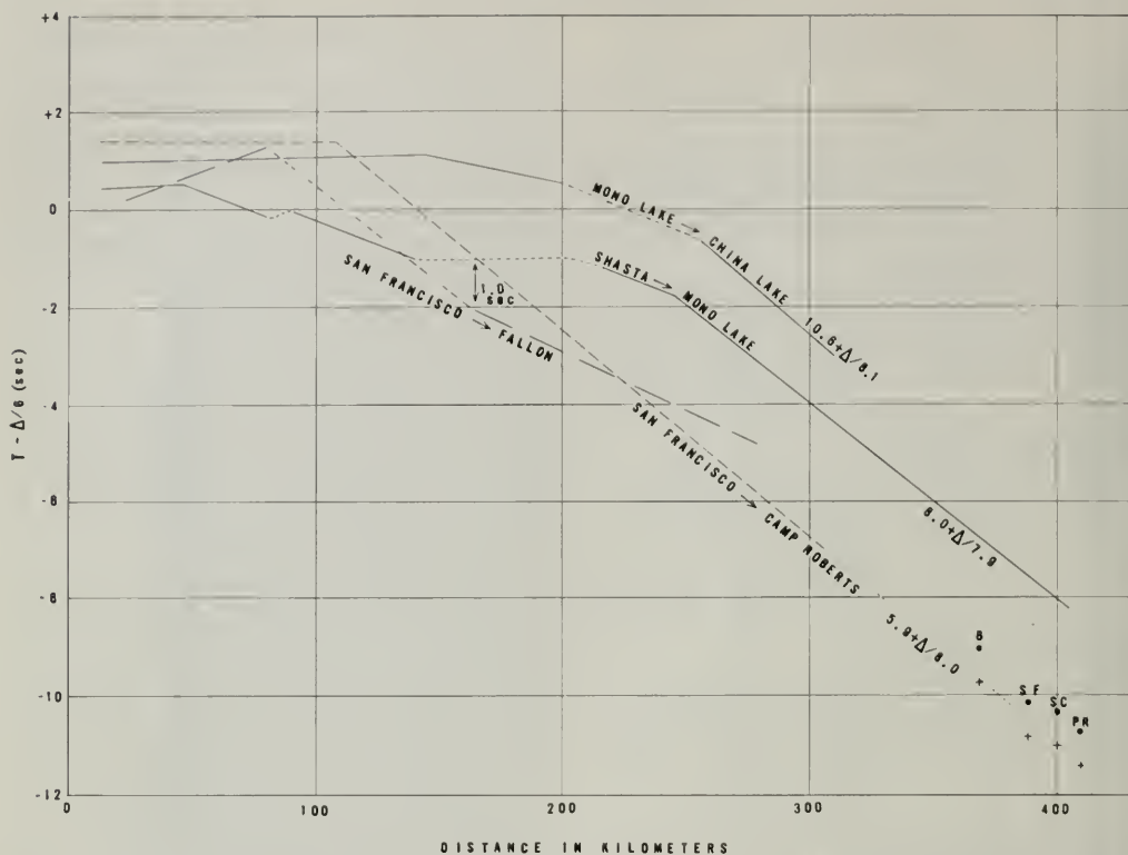
Figure 4. Reduced traveltime curves of first arrivals on selected profiles shown on figure 1. T - \Delta/6 , where T is traveltime in seconds and \Delta is shot to receiver distance in kilometers, is plotted against \Delta . Uncorrected reduced traveltimes versus distance from SHOAL to seismograph stations near the San Francisco Shotpoint are shown as solid circles (B, Berkeley; SF, San Francisco; SC, Santa Cruz; and PR, Point Reyes). After correction for diffraction around the Sierra Nevada root (fig. 5), they are shown as crosses.
