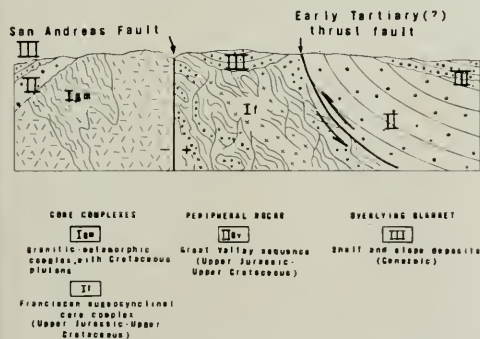
Figure 2. Schematic section across Coast Ranges, not drawn to scale, showing the relations of the principal rock assemblages.
