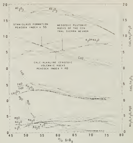
Figure 5. Silica variation diagram for Cenozoic volcanic rocks of the alkalic Stanislaus Formation (solid lines), the calc-alkaline volcanic rocks of the Mehrten Formation (dashed lines), and calc-alkaline Mesozoic plutonic rocks of the central Sierra Nevada (dotted lines). The principal sources of analytical data are from Curtis (1951), Halsey (1953), Slemmons (1953), and Washington (1917).
