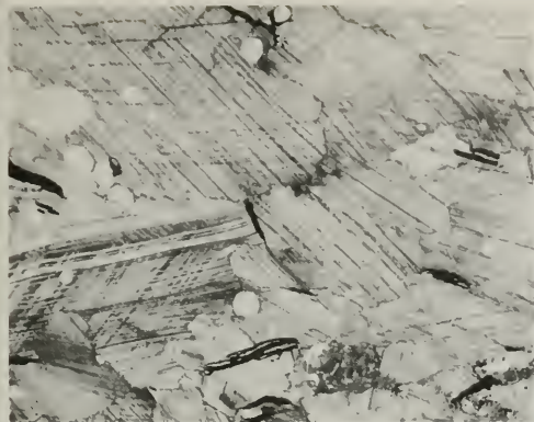
Photo 2. Photomicrographs of Sur marble. Left, strongly twinned calcite grains with black graphite tablets and equidimensional, white grains of apatite and K-feldspar. Right, recrystallized fine-grained calcite with large relics of K-feldspar (white), clinopyroxene (lined), and altered meionitic scapolite (dark gray). Views are 6 mm across. Plane polarized light.
