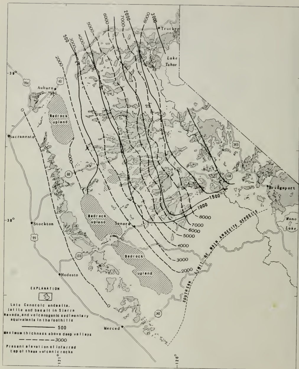
Figure 4. Map showing distribution of late Cenozoic andesite, latite, basalt, and Pliocene rhyolite. The approximate maximum original thickness above the deeper pre-andesite valleys is indicated by the solid isopachs. The dashed contours denote the approximate present elevation of the inferred top of these volcanic rocks. In addition to the main bedrock uplands of the foothill belt, there were probably other areas at higher elevations on which little or no volcanic rock was deposited.
