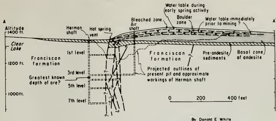
Figure 5. Geologic section through the Sulphur Bank mine area along line A-A', of figure 4.
