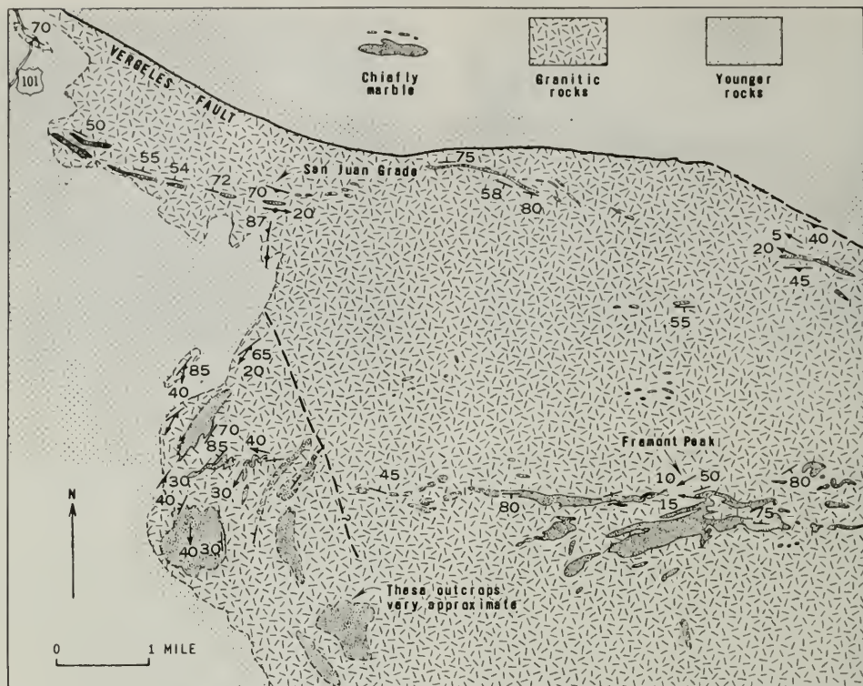
Figure 8. Map of north end of Gabilan Range, with marble relics suggesting a large fold around which earlier lineations have been rotated. Chiefly from maps of Allen (1946), Bowen and Gray (1959), and Santa Cruz sheet of the Geologic Map of California (Jennings and Strand, 1958), with additions by the writer.
