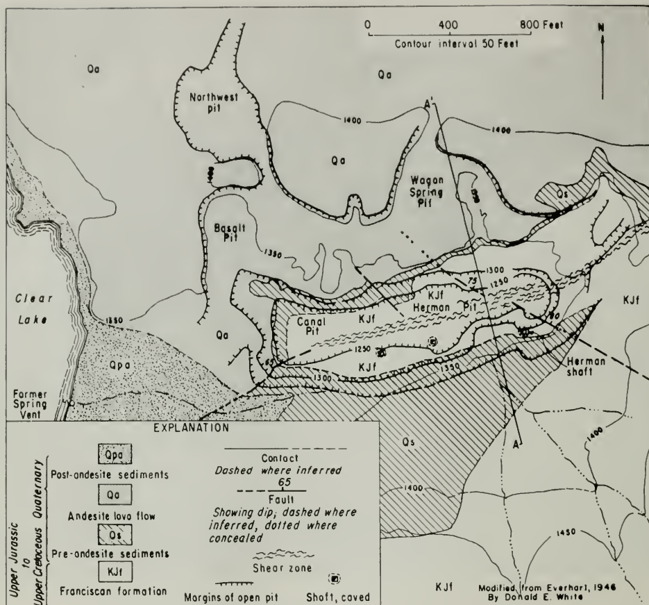
Figure 4. Geologic map of the Sulphur Bank mercury mine area.
