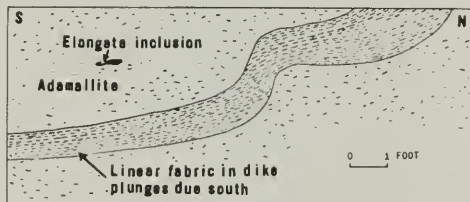
Figure 2. Granitic dike with strongly linear fabric as exposed in vertical cut on Block Mountain road, 1½ miles northwest of Navajo Road summit. The dike strikes due west.
