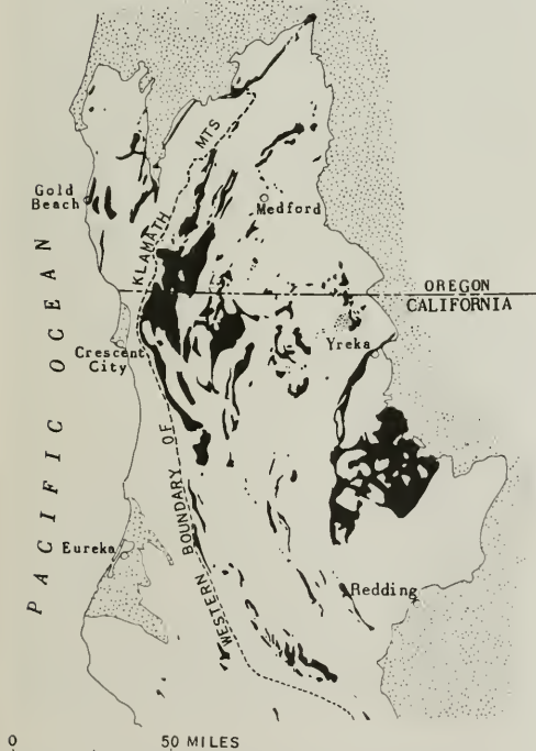
Figure 5. Map showing arcuate distribution of ultramafic rocks in Klamath Mountains of California and Oregon. Ultramafic rocks shown as solid black areas. Mantle of Cenozoic rocks shown as stippled areas.
