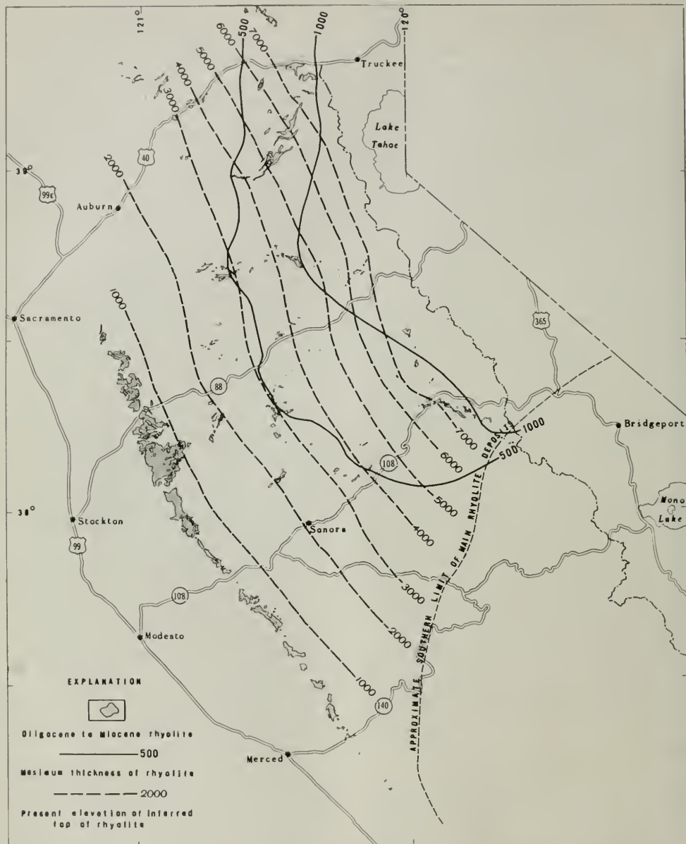
Figure 2. Map showing distribution of Oligocene to Miocene rhyolites of the central Sierra Nevada, with solid contours denoting their approximate maximum original thickness. The dashed contours indicate the approximate elevation of the inferred top of the rhyolites. The deep and repeated dissection of the rhyolites makes the indicated isopachs minimal values for the thickness in deeper valleys. Although there may have been several areas of nondeposition between some of the southwest-trending channels of maximal thickness, the isopachs and contours of elevation are projected between the main channels.
