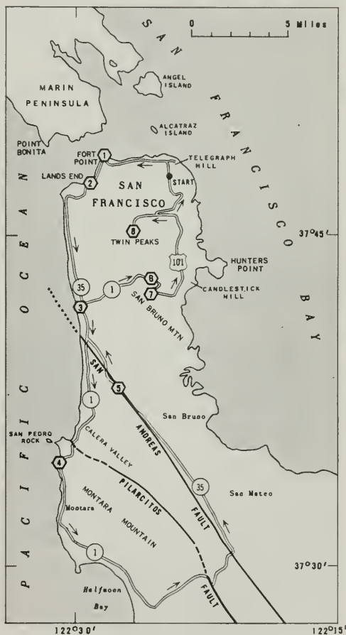
Figure 1. Index map of San Francisco peninsula showing route of field trip; stops in road log indicated by numbers in hexagons.
