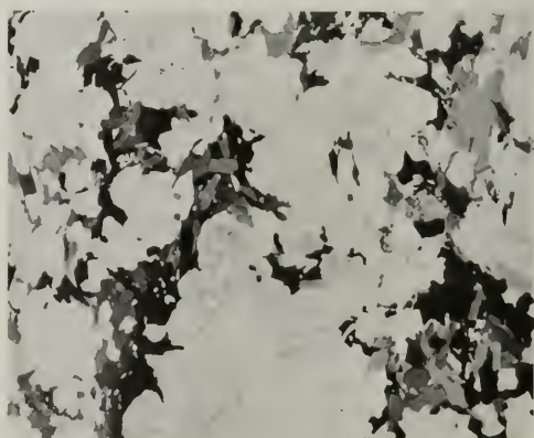
Photo 1. Photomicrograph of typical allotriomorphic quartz diorite of Junipero Serra area, showing clustered biotite grains. View is 12 mm across. Plane polarized light.
