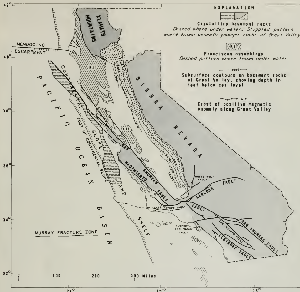
Figure 2: Principal structural features of the California continental margin modified from Bailey, Irwin, and Jones (1964). Offshore crystalline basement rock areas are after Uchupi and Emery (1963) and Curry (1965).
