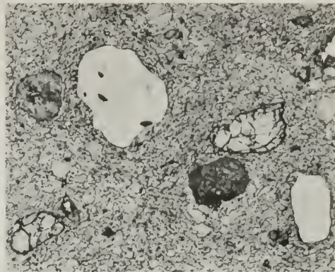
Photo 2. Photomicrographs of Sur marble. Left, strongly twinned calcite grains with black graphite tablets and equidimensional, white grains of apatite and K-feldspar. Right, recrystallized fine-grained calcite with large relics of K-feldspar (white), clinopyroxene (lined), and altered meionitic scapolite (dark gray). Views are 6 mm across. Plane polarized light.
