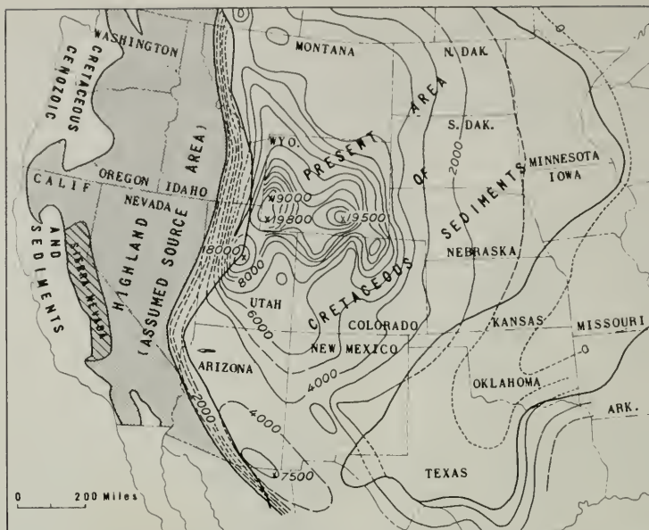
Figure 3. Map of the western United States showing the general distribution of land and sea during the Late Cretaceous. Isopachs show thickness of Cretaceous sediments in the Rocky Mountain geosyncline. Modified from two illustrations by Gilluly (1963).
