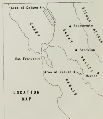
Figure 3. Representative columnar sections of "peripheral rocks" of late Mesozoic age.
