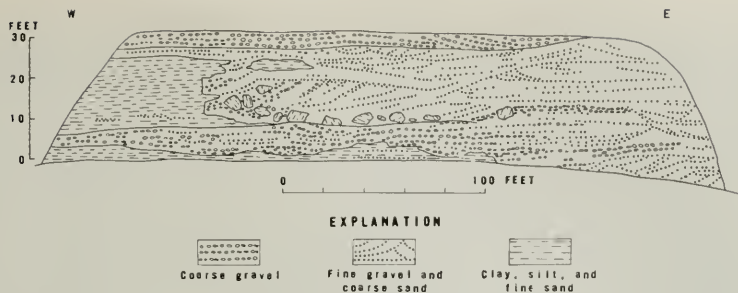
Figure 8. Sketch from photograph of roadcut 1 mile west of North Columbia, Nevada County, California, showing local unconformities probably caused by lateral migration of an aggrading stream into bodies of overbank silt on its floodplain. Vertical exaggeration 2 X.
