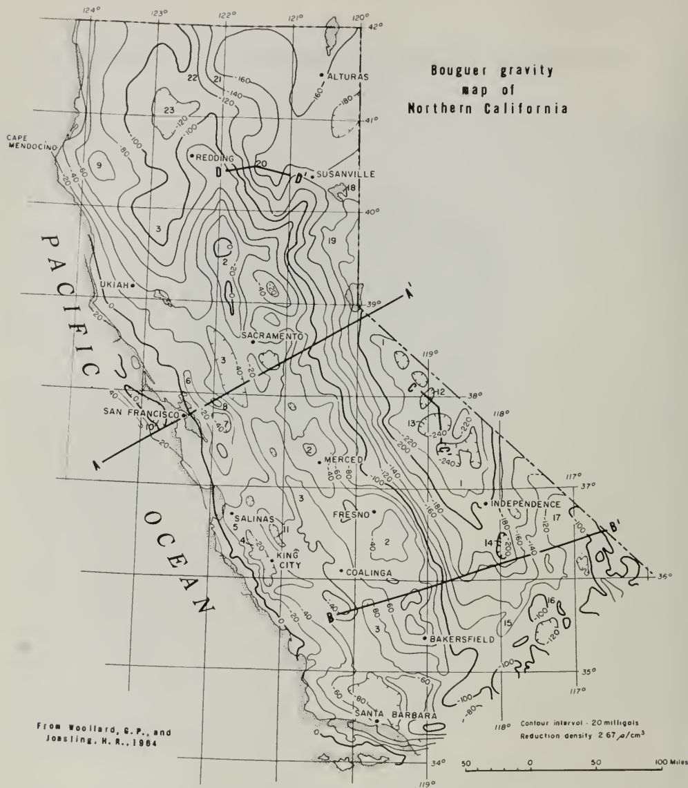
Figure 1. Bouguer gravity map of northern California (after Woollard and Jaesting, 1964).
