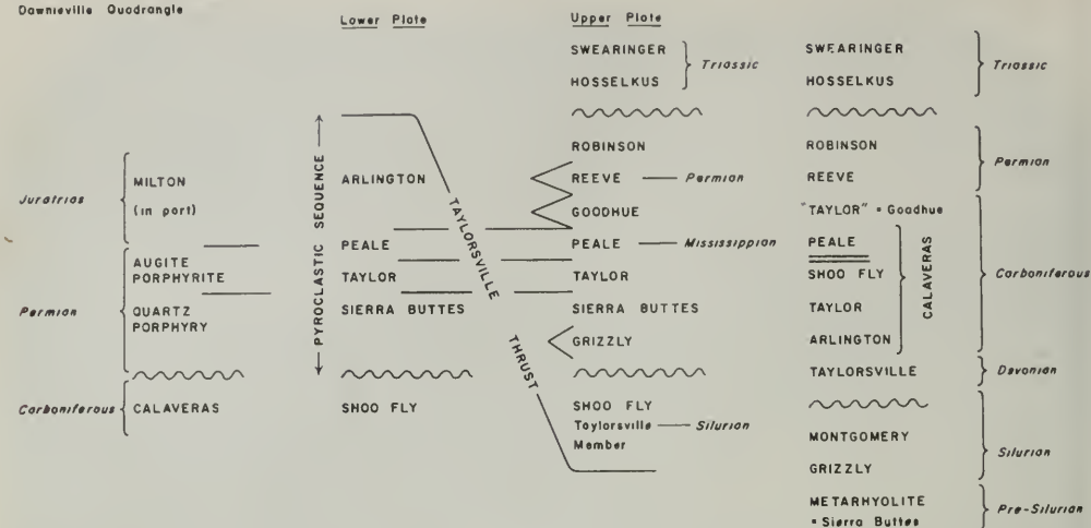
Figure 3. Pre-Jurassic correlation diagram for the Taylorsville area. Diller's column (on right) is modified in that his eastern belt of Taylor Meta-Andesite is inserted between his Peale and Reeve as demanded by his map relations, and his Robinson and Reeve Formations are indicated as Permian as emended by Thompson and others (1946). Turner considered his augite porphyry and quartz porphyry to be Jurassic in age, but they are shown as Permian as emended by Wheeler (1939).
