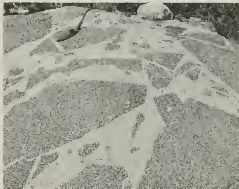
Photo 3. Intrusive breccia. A (left)—Fragmentation of metamorphic rock by granitic magma. B (right)—Fragmentation of early quartz diorite by later quartz monzonite.
