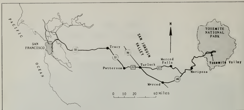
Figure 1. Index map showing route of field trip from San Francisco to Yosemite Valley.
