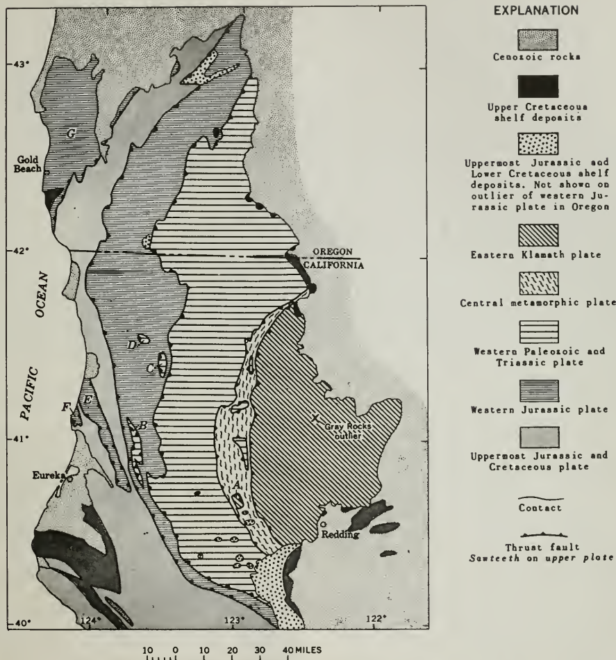
Figure 7. Principal postulated thrust plates of the Klamath Mountains and adjacent Coast Ranges. Thrust outliers are indicated by letter symbol: A, Oregon Mountain; B, Willow Creek; C, Prospect Hill; D, Flint Valley; E, Redwood Mountain; F, Patricks Point; and G, southwestern Oregon.
