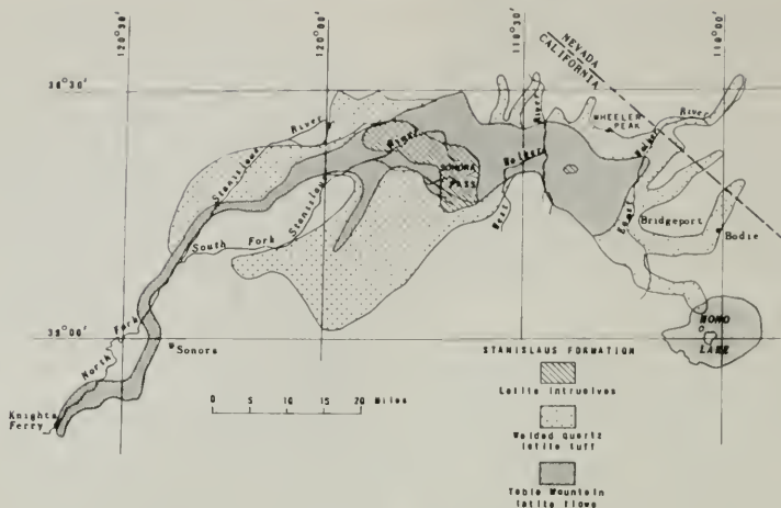
Figure 3. Map showing inferred original distribution of the Stanislaus Formation, and the original distribution of the Table Mountain Latite Member and the welded biotite-quartz latite tuffs of the Eureka Valley Member. The volcanic centers for the Table Mountain Member are in the area indicated by the diagonal pattern near Sonora Pass, and a possible intrusive source for the Eureka Valley Member is similarly indicated about 15 miles east of Sonora Pass.
