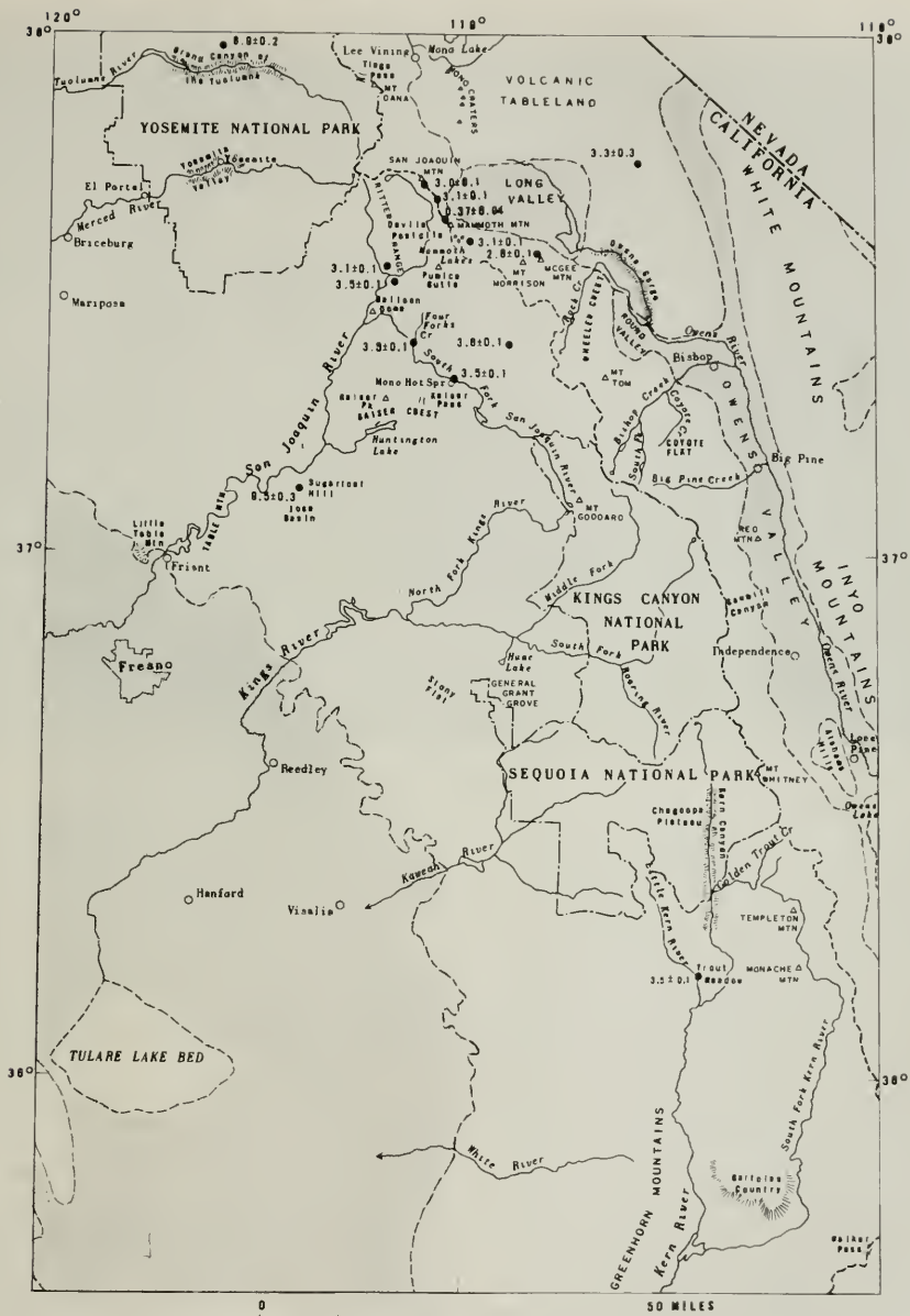
Figure 6. Map showing localities in southern Sierra Nevada mentioned in text, and locations of Cenozoic volcanic rocks in southern Sierra Nevada dated by the potassium-argon method (from Dalrymple, 1963; 1964a, b; Doell, Dalrymple, and Cox, 1966).
