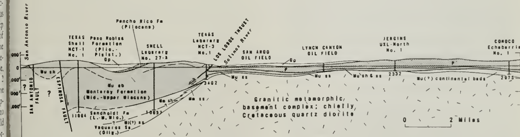
Figure 9. Geologic cross section through an area near San Ardo, west of the San Andreas fault and the area shown in figure 8. Modified from Plate 2 of A.A.P.G.—S.E.P.M., Guidebook to the Geology of Salinas Valley and the San Andreas fault, 1963, by H. Waldron and E. A. Gribb.
