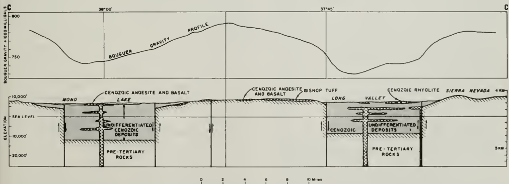
Figure 4. Bouguer gravity profile along C-C', figure 1, across Mono Basin and Long Valley, showing assumed subsurface structure (after Pakiser and others, 1964, fig. 9).
