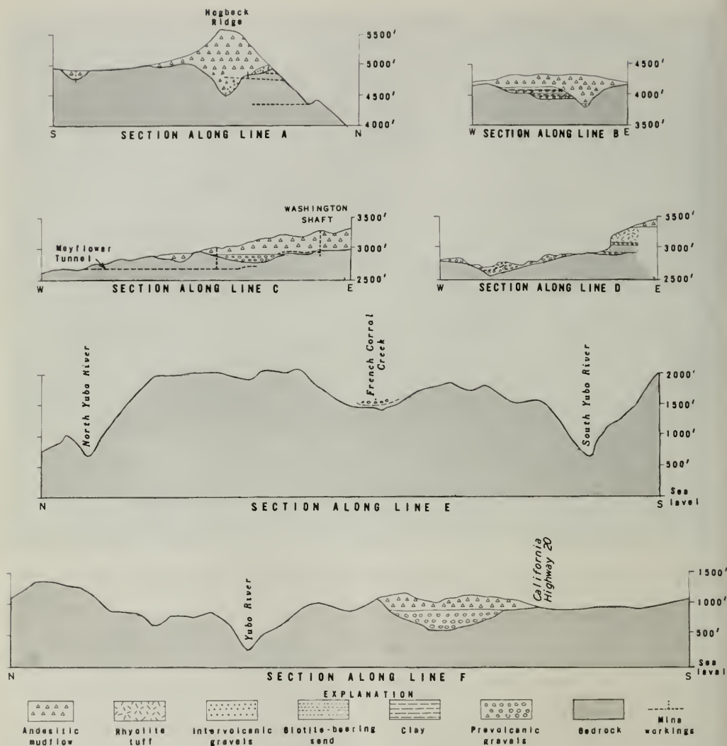
Figure 9. Cross sections of the channel of the Tertiary Yuba River along lines shown on figure 12. Sections A, B, and C from Ross E. Browne, 1890; section D from MacGinitie, 1941, p. 19; sections along E and F constructed from 1:24,000 Smartsville and French Corral quadrangles with geology by Wahrhaftig. Vertical exaggeration 2 X.
