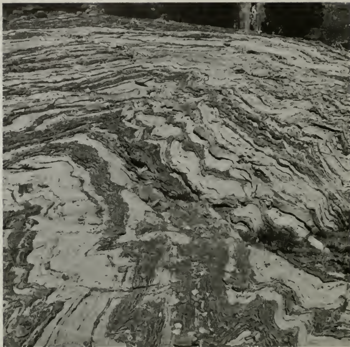
Photo 1. The metamorphosed strata of the Sierra Nevada are complexly folded. A (above)—Gently plunging fold in hornfels and marble. B (below)—Chevron folds in tuffaceous slate.
