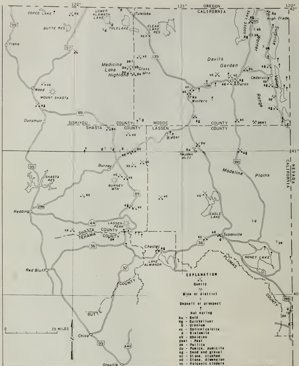
Figure 2. Map showing the location of hot springs and deposits of economic mineral commodities in northeastern California.
