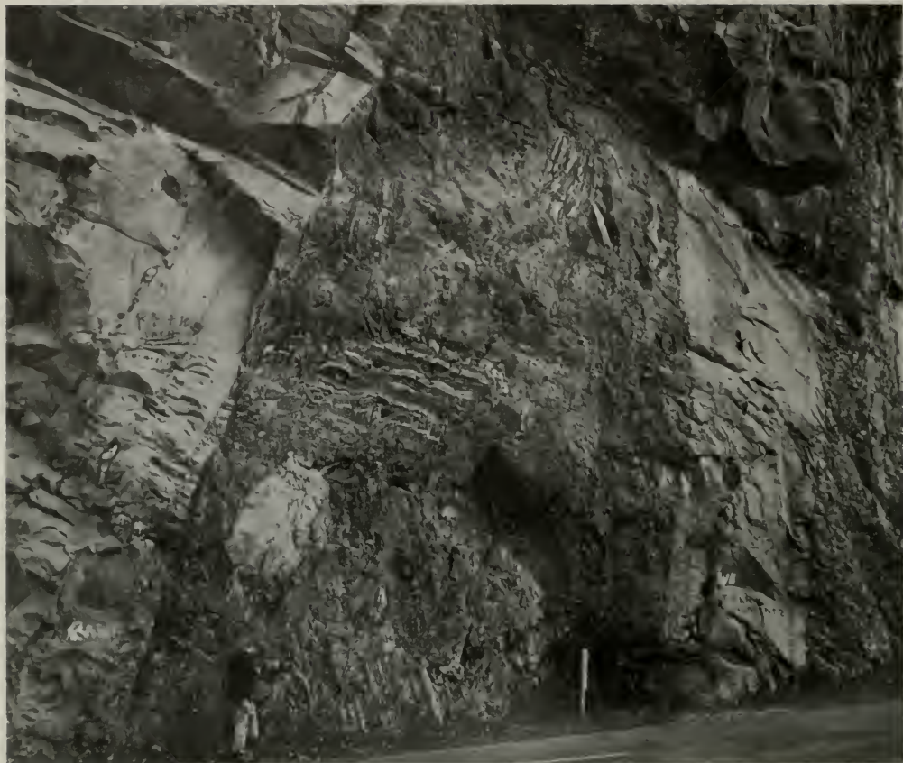
Photo 2. Pebbly mudstone with displaced blocks of interbedded sandstone and shale, at base of Venado Formation (Late Cretaceous, Turonian) near Monticello Dam on State Highway 128, Capay quadrangle.
