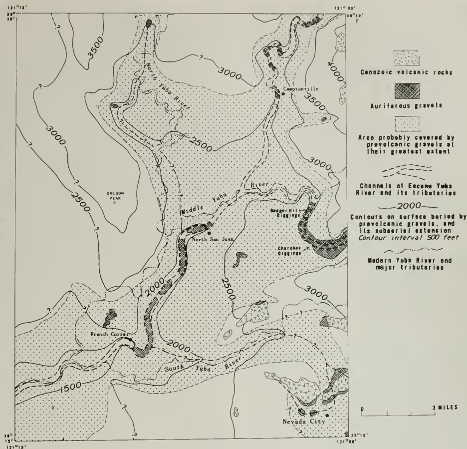
Figure 7. Map of Nevada City quadrangle, showing auriferous gravel deposits, channels of Tertiary Yuba River, probable original extent of gravels, and topography on surface buried by the Cenozoic rocks. Data from Whitney, 1880; Lindgren, 1911, and Smartsville Folio; and original reconnaissance survey. For location of quadrangle see figure 5.
