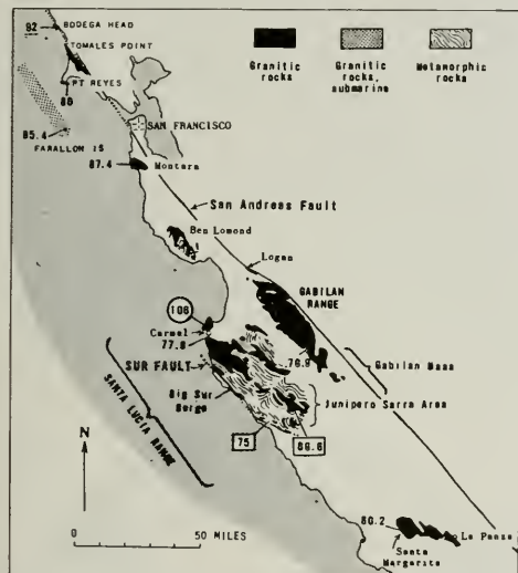
Figure 1. Index map of a central part of the Coast Ranges showing principal exposures of Salinian granitic and metamorphic rocks. Numbers are absolute ages in millions of years; those unmarked are from Curtis, Evernden, and Lipson (1958) recalculated to 1965 values of decay rates; the circled 106 is a nonisotopic Th-Pb age for monazite from Pacific Grave (Hutton, 1959, p. 20); the numbers in rectangles are unpublished K-Ar ages determined by John Obradovich (see table 1), and the underlined 92 is an unpublished K-Ar age determined by R. W. Kistler (see table 1). Submarine outcrop from Uchupi and Emery, 1963.
