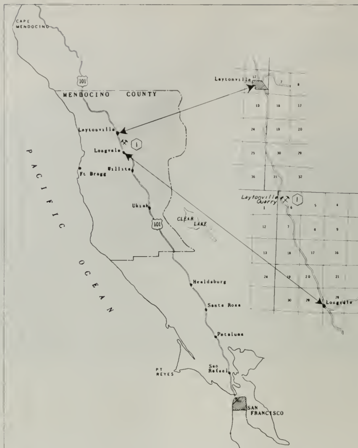
Figure 1. Map showing route of field trip from San Francisco to the Laytonville quarry.
