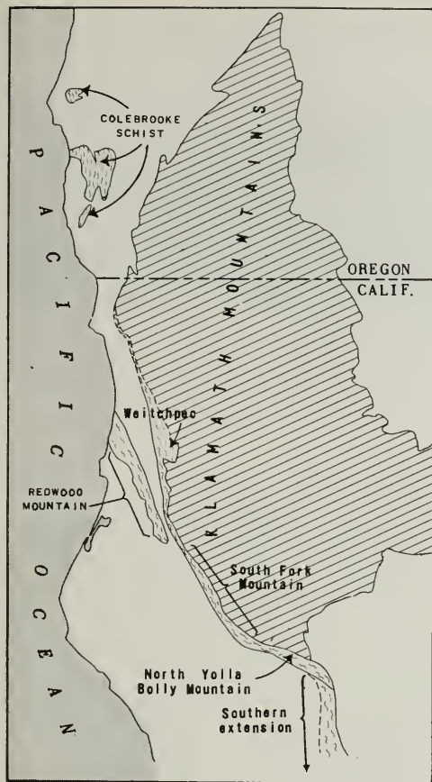
Figure 4. Distribution of South Fork Mountain and related schists. Southern extension (after Ghent, 1965, and Blake, 1965) is an area of rocks considered at least in part equivalent to schist of South Fork Mountain.
