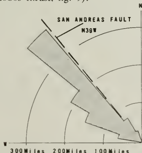
Figure 10. Diagram showing relation of fold trends to strike of San Andreas fault in area between Santa Maria and Coalinga. Predominant trend is N. 40^{\circ} - 50^{\circ} W., making only a small angle with the San Andreas fault. Based on cumulative lengths of fold axes lying within 10^{\circ} -degree intervals of azimuth; measurements from part of tectonic map by Reed and Hallister, 1936.
