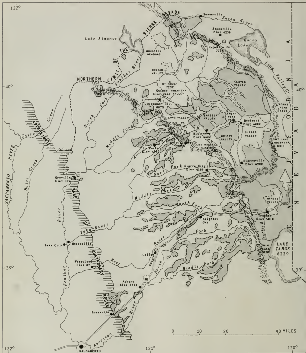
Figure 2. Map of the northern Sierra Nevada, showing the distribution of Miocene and Pliocene rocks, and location of lines of cross sections shown in figure 3.
