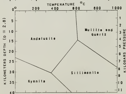
Figure 4. Fields of stability of andalusite and its polymorphs according to Waldbaum (1965). (Modified slightly.)
