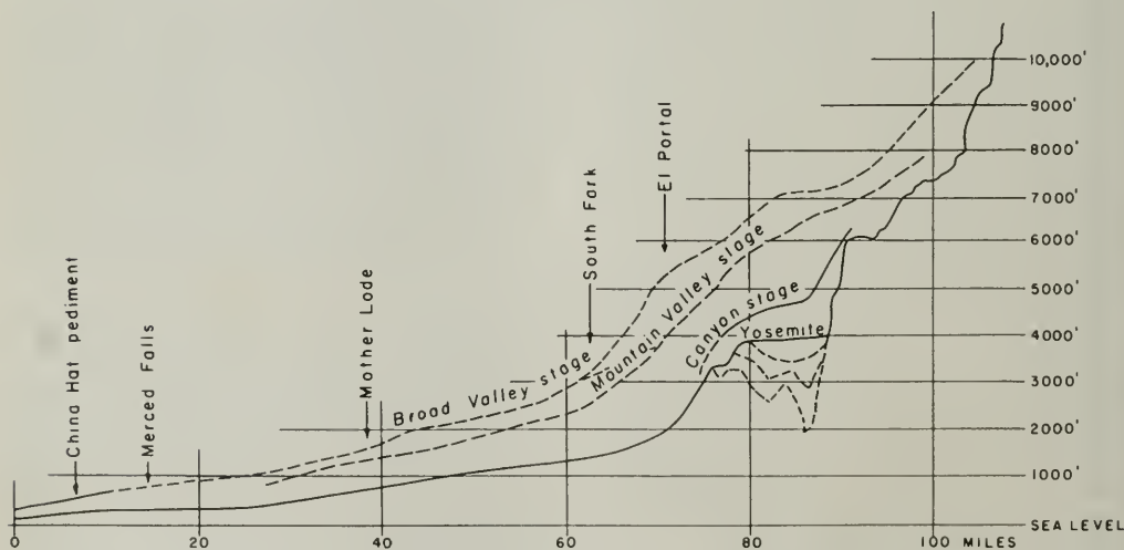
Figure 15. Longitudinal profile of the Merced River (after Hudson, 1960, p. 1551—reproduced from Wahrhaftig, 1962, fig. 3, p. 37).
