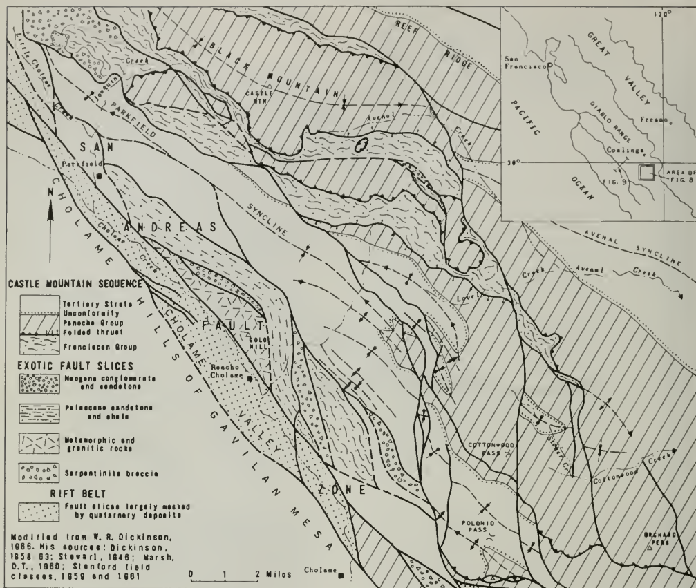
Figure 8. Geologic map of an area east of Cholame Valley in the southern part of the Coast Ranges (after W. R. Dickinson).
