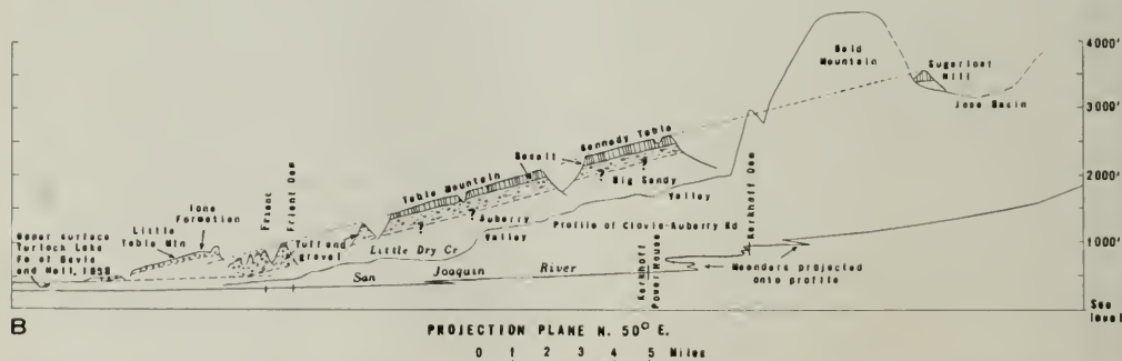
Figure 13. Projections of two volcanic table mountains of the western Sierra Nevada. A. Projection of Tuolumne Table Mountain onto a vertical plane striking N. 40° E. Geology modified from Taliaferro and Solari, 1949; Eric and others, 1955; and Big Trees Folio. B. Projection of Little Table Mountain and the basalt of Table Mountain on the San Joaquin River onto a vertical plane striking N. 50° E. Geology modified from Macdonald, 1941, and original surveys. For location of projection planes see figure 10. Vertical exaggeration about 10 X.
