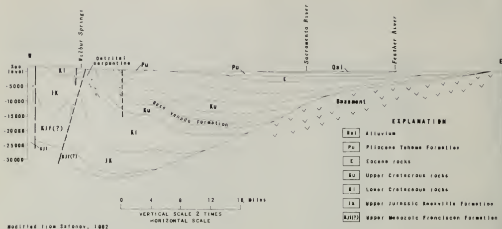
Figure 3. Generalized E-W section across the Sacramento Valley from near Wilbur Springs to a point a few miles east of Marysville. Modified from Safonov (1962).
