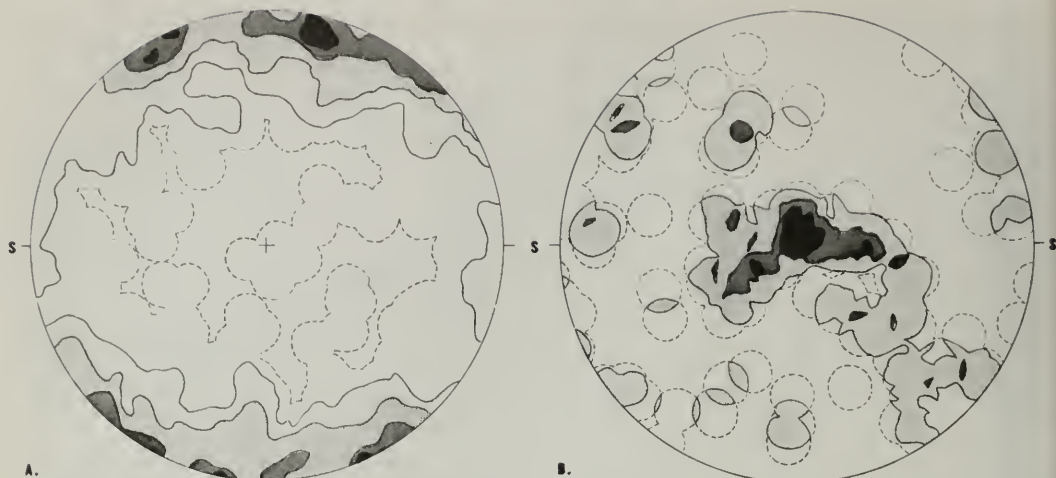
Figure 7. Petrofabric diagrams of quartz diorite sectioned approximately at right angles to megascopic lineation that is parallel to first fold axes of Sur series. A, Pales to cleavage in 500 biotite grains, corrected for Schnitteffekt ; contours at 4, 3, 2, 1, and 0.2 percent per 1 percent of area. B, X optic axes (approximately parallel to a crystallographic axes) of 100 andesine grains in same thin section as A; contours at 4, 2, and 1 percent per 1 percent of area. SS, biotite foliation. Sample from San Antonio River narrows, 7\frac{1}{2} miles southeast of Junipero Serra Peak.
