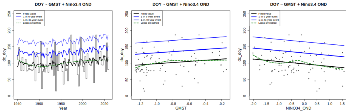
Figure 3.9: Day of hydrologic year (days since 1 September) on which the drought season ends (DC-DOY) in ERA5, with fitted linear trends. The heavy black line indicates the location of the distribution; blue lines indicate the 6-year and 40-year expected return level; the green dashed line is a nonparametric Loess smoother. At the time of writing the 2024-25 dry season was still ongoing, so there is no observed value. (a) Fitted trend over time; (b) DC-DOY as a function of GMST anomaly from 2025, in °C, with Niño3.4 covariate fixed at its mean level; (c) DC-DOY as a function of OND Niño3.4 index, with GMST fixed at its mean level.
