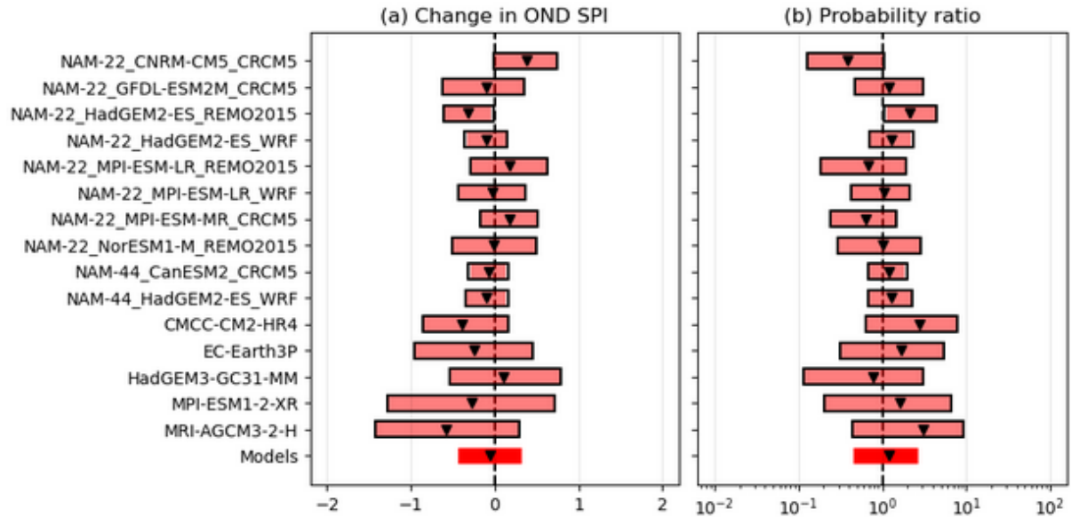
Figure 3.8: As Figure 3.7, synthesising changes in SPI-OND between the current climate and a 1.3°C warmer climate (that is, a climate that is 2.6°C warmer than preindustrial).
