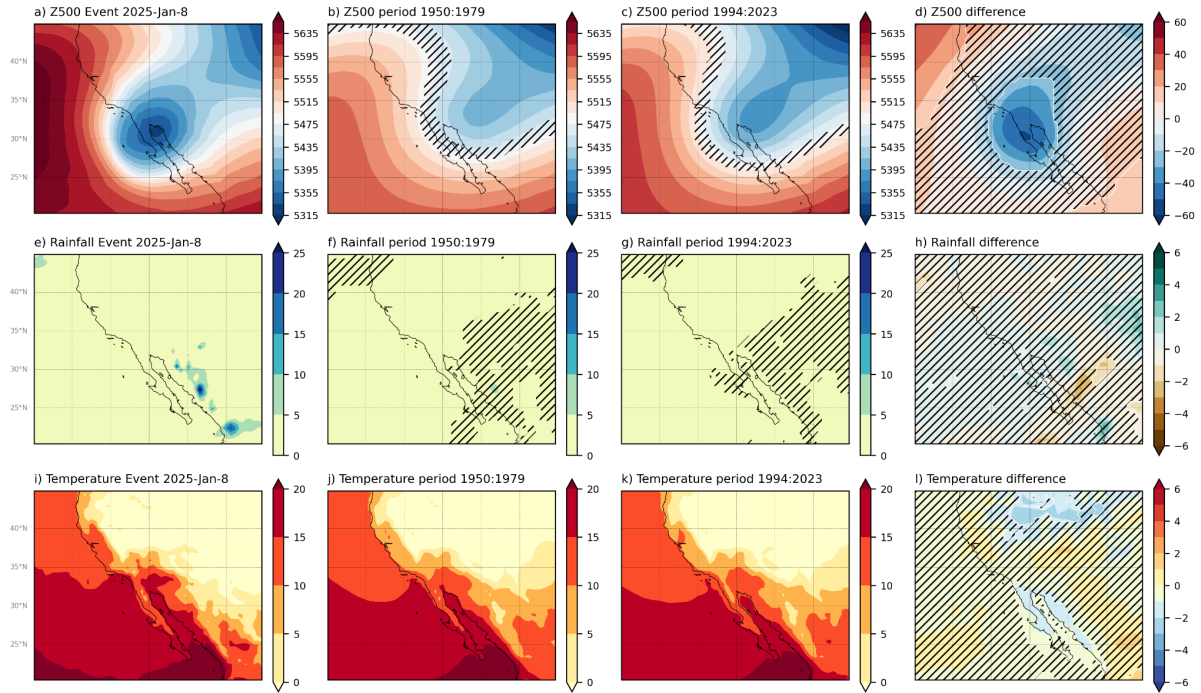
Figure 4.2: Changes in atmospheric analogues. (a) 500hPa geopotential height field (m) for the event, 8 Jan 2025. b) Composite of the top 27 analogue days from the past period, 1950-1979. c) Composite of the top 27 analogue days from the present period, 1994-2023. d) Difference between the composites of past and present (present minus past). e-h) as in a-d for the rainfall field (mm). i-l) as in a-d for the 2m temperature field (°C). Z500 used to identify analogues in all plots. Hashing signifies regions where the signal is not significant based on a two-sided t-test.
