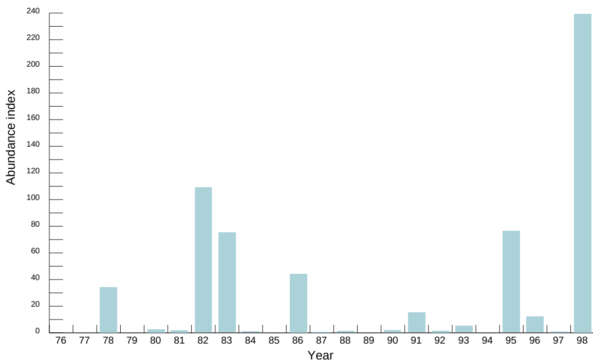
Figure 3-3 Young-of-the-Year Splittail Abundance Index, Fall Midwater Trawl, 1976 through 1998
