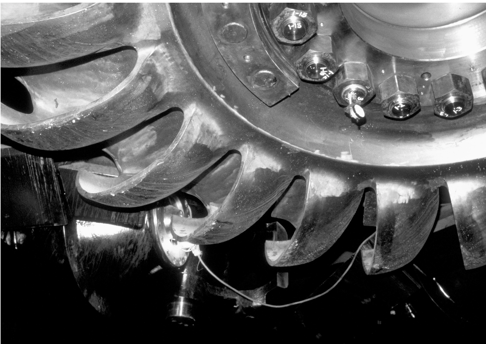
Construction of the interior of Devil Canyon Powerplant
