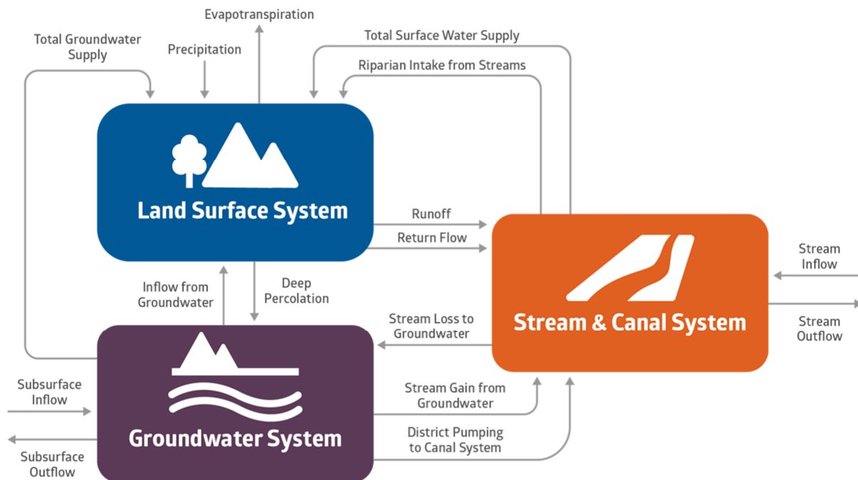
Figure 7: Modesto Model Water Budget Flow Diagram
