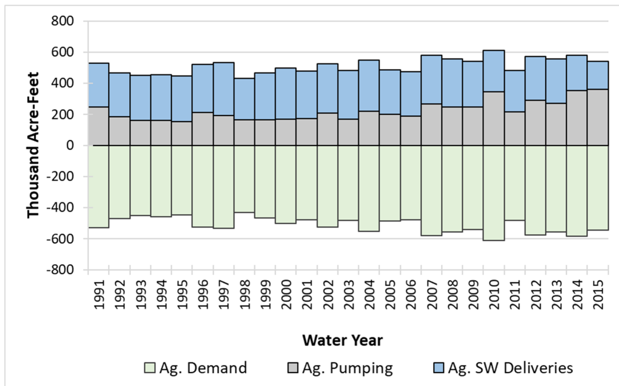
Figure 10: Modesto Subbasin Annual Agricultural Land and Water Use Budget
