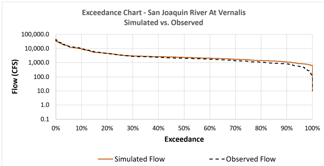
Figure 29: Streamflow Exceedance Probability for the San Joaquin River at Vernalis
