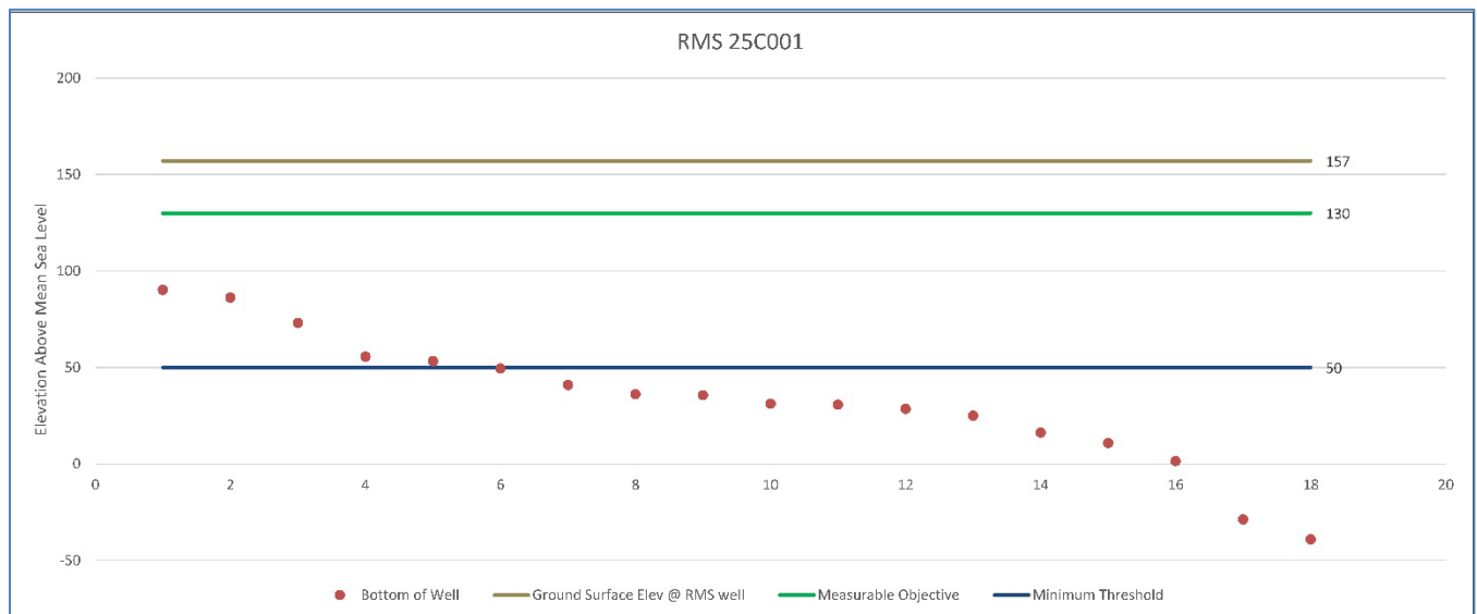
Figure 3-3: Graph Showing Graphing Method Used to Establish MTs for Each RMS Well. Red dots represent bottom elevation of each domestic well within the polygon associated with the RMS well (example is for well 25C001M in Vina North) relative to ground surface elevation at the RMS well
