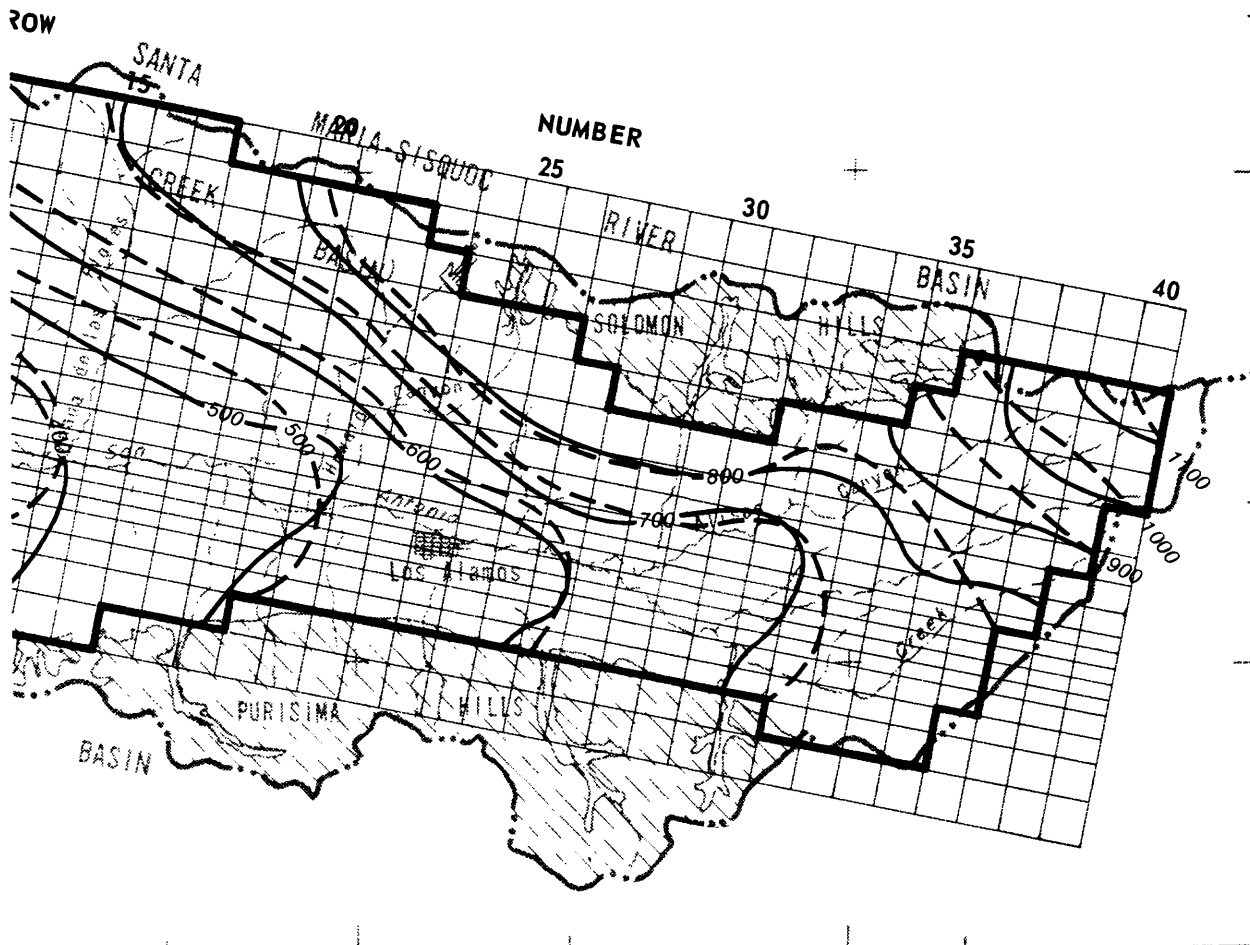
Consolidated rock boundaries from K. S. Muir (1964)
