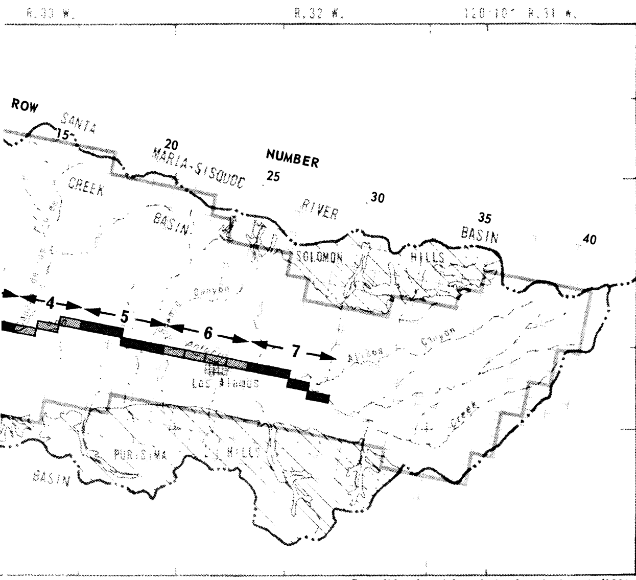
Consolidated-rock boundaries from K. S. Muir (1964)
