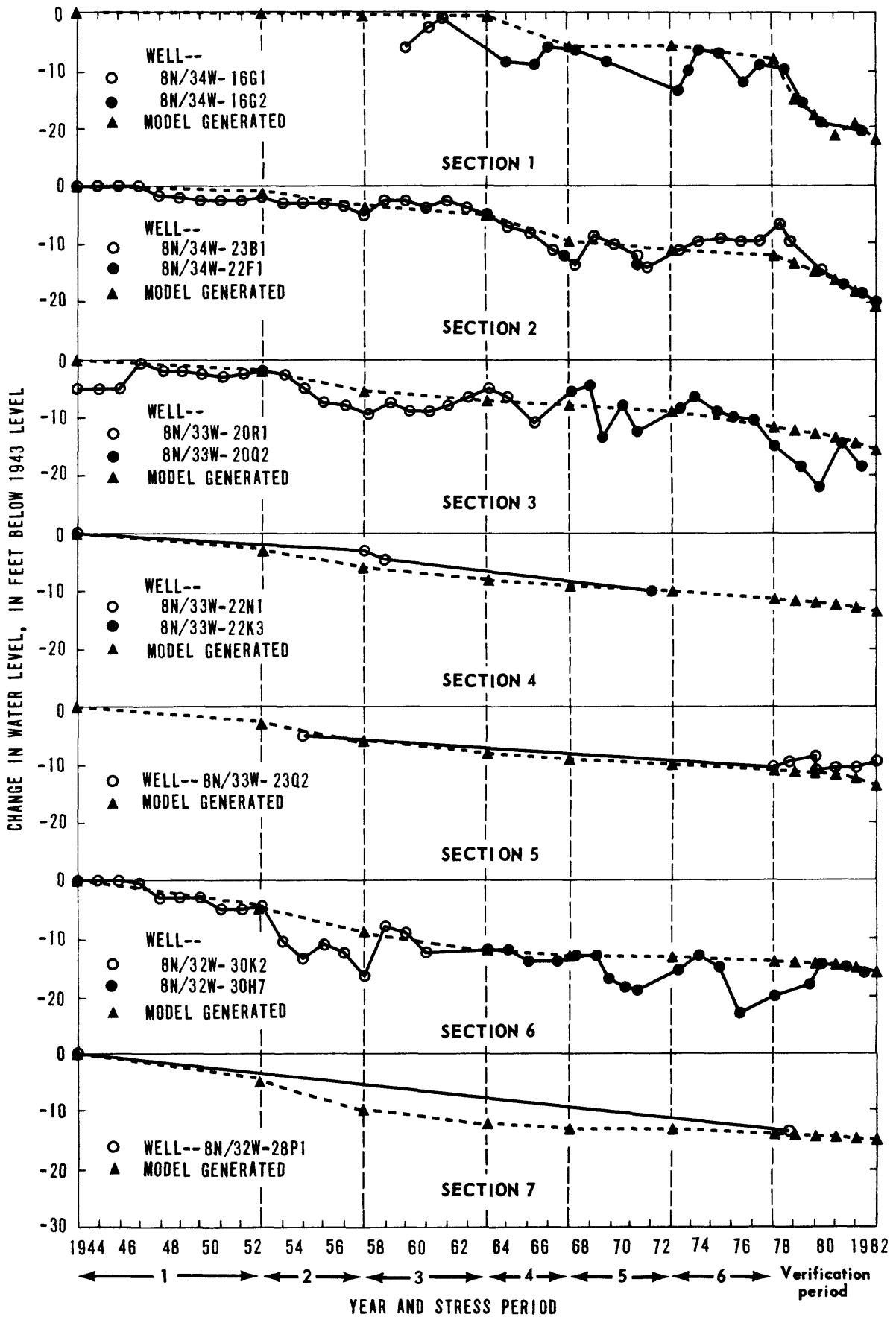
FIGURE 11.—Hydrograph showing comparison of model-generated and historical measured water levels.
