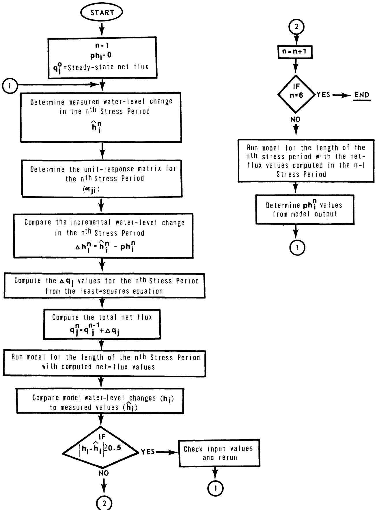
FIGURE 13.—Flow chart of the net-flux calibration.
