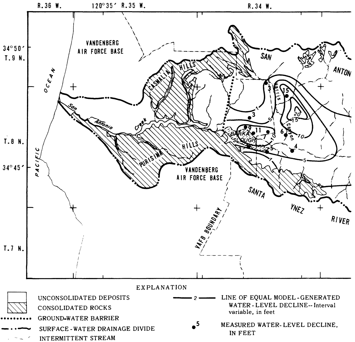
FIGURE 16. -- Comparison of measured and model-generated water-level decline, 1977-82.
