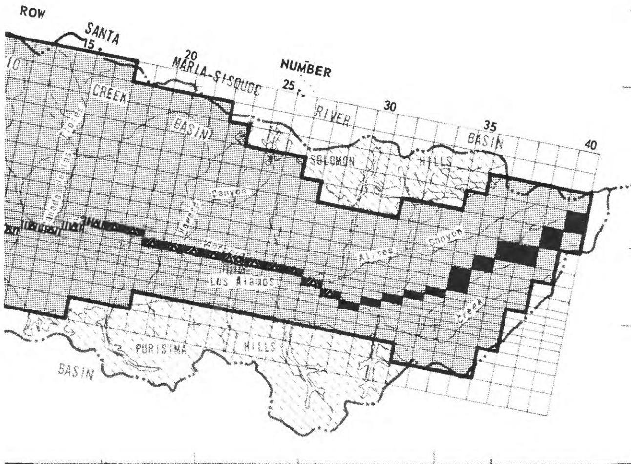
Consolidated-rock boundaries from K. S. Muir (1964)
