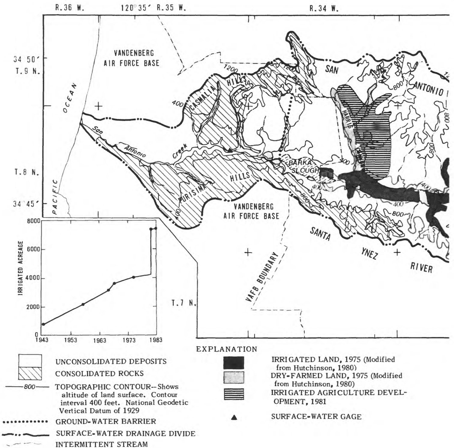
FIGURE 3.-- Topography and land use in the San Antonio Creek valley.
