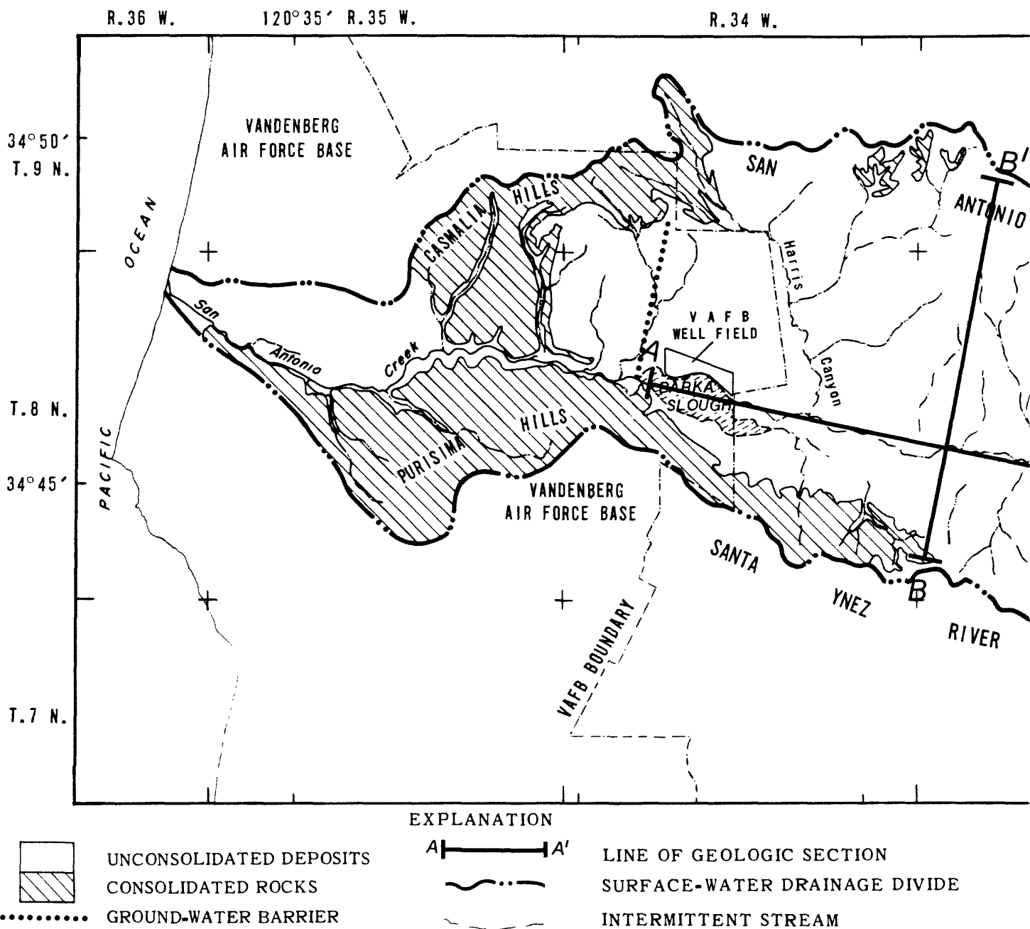
FIGURE 1.--Location of geologic sections and location and general features of San Antonio Creek valley.
