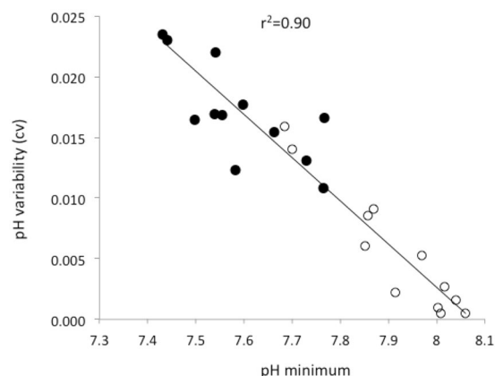
Figure 2. Increase in pH variability (coefficient of variability) as a function of pH minimum across surface ocean datasets from present study (solid circles) and from a cross-biome survey 13 (open circles) that includes representation from tropical, temperate, and polar surface ocean sites. Three sites that are strongly influenced by unique local conditions (an estuary, a volcanic CO 2 vent and a groundwater discharge site) are excluded.
