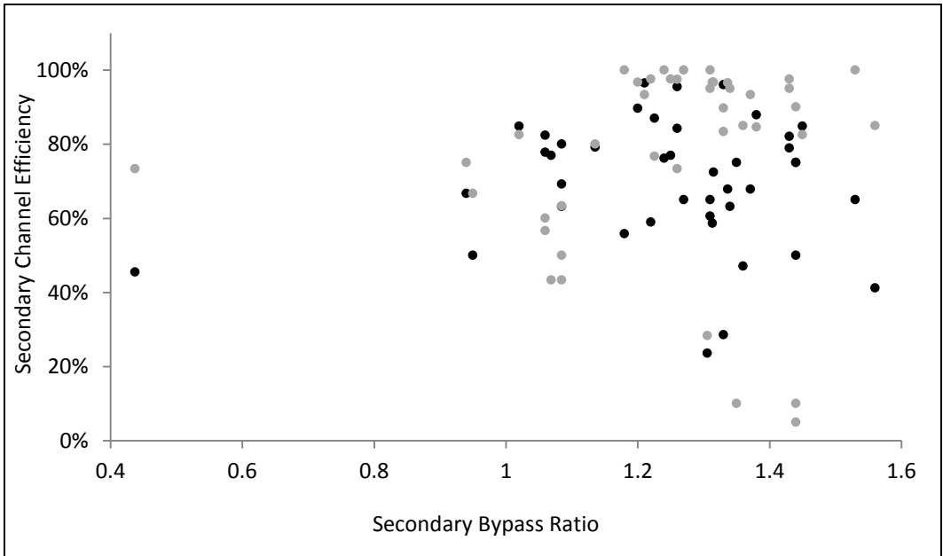
Figure A4-2.—Effects of secondary channel bypass ratio on secondary channel efficiency (black circles) and secondary channel participation (grey circles) of adult delta smelt ( Hypomesus transpacificus ) at Bureau of Reclamation’s Tracy Fish Collection Facility (Byron, CA).
