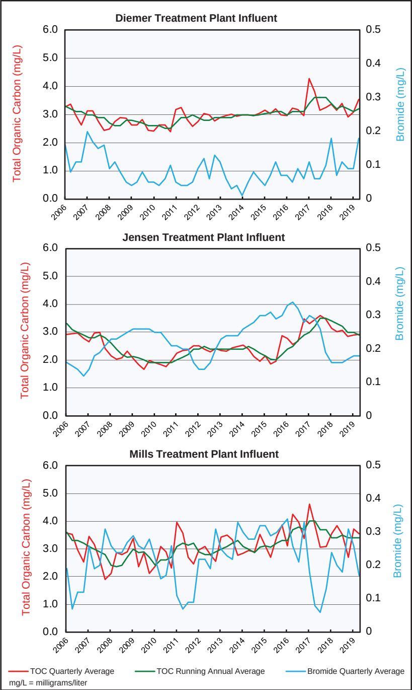
Figure 4-5. Total Organic Carbon (TOC) and Bromide Levels in Treatment Plant Influent, 2006 to 2019
