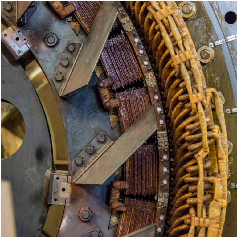
Valley View hydroelectric plant generator, rotor and windings during plant refurbishment.
