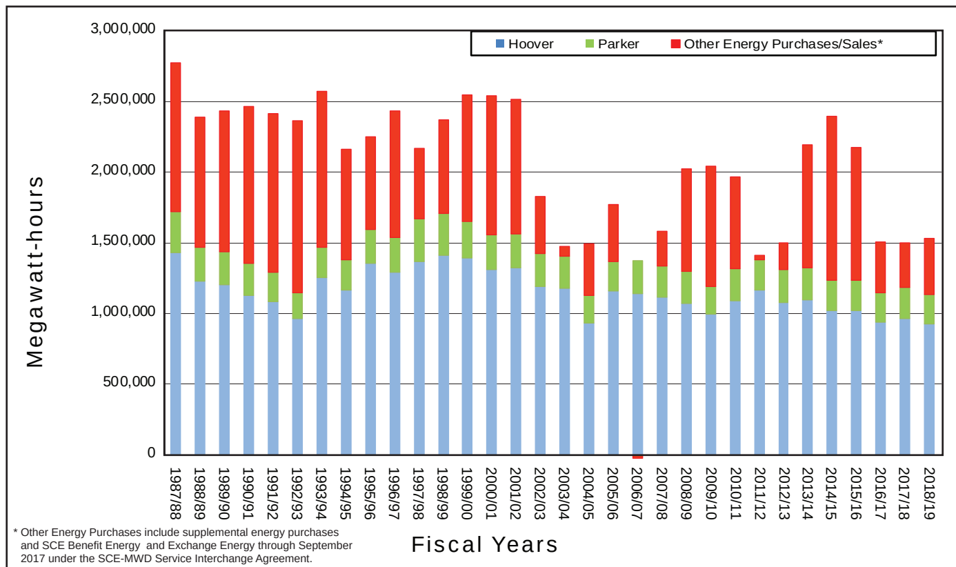
Figure 4-12. CRA Energy Mix, Fiscal Years 1987/88 to 2018/19
