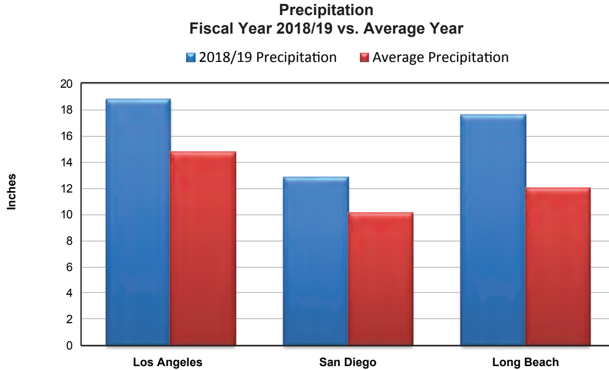
Figure 3-6. Precipitation
