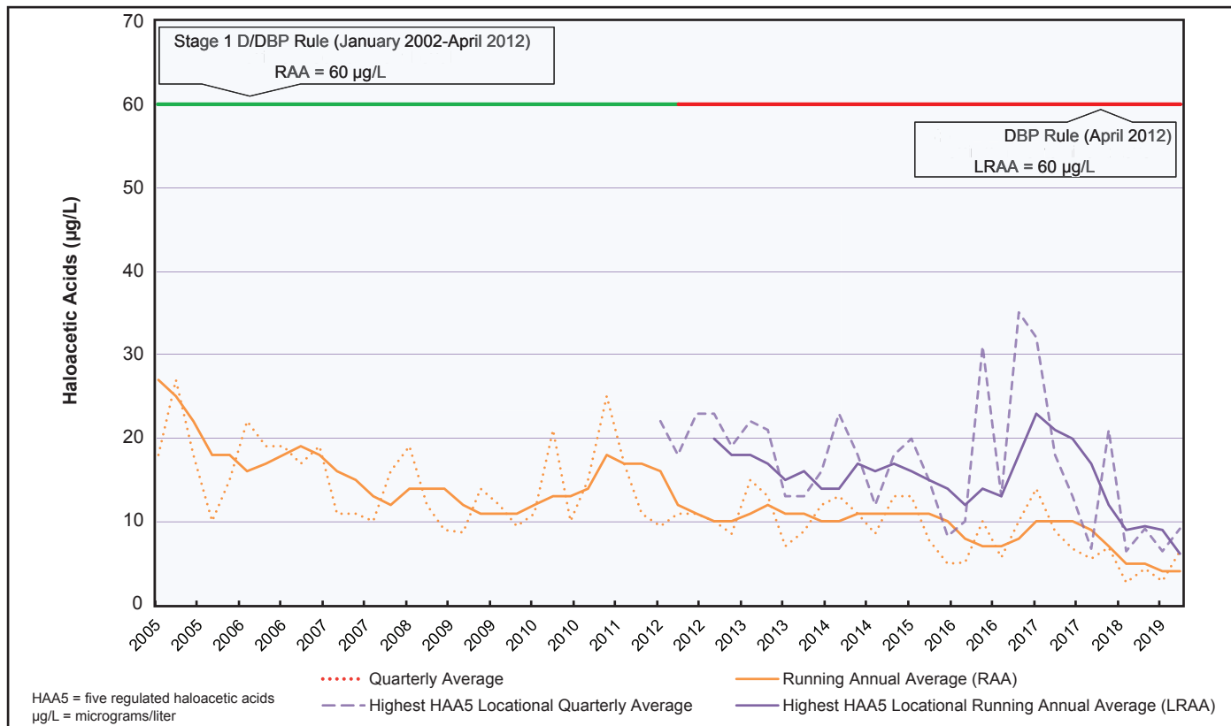
Figure 4-4. Haloacetic Acids Throughout the Distribution System, Quarterly and Running Annual Averages, 2005 to 2019
