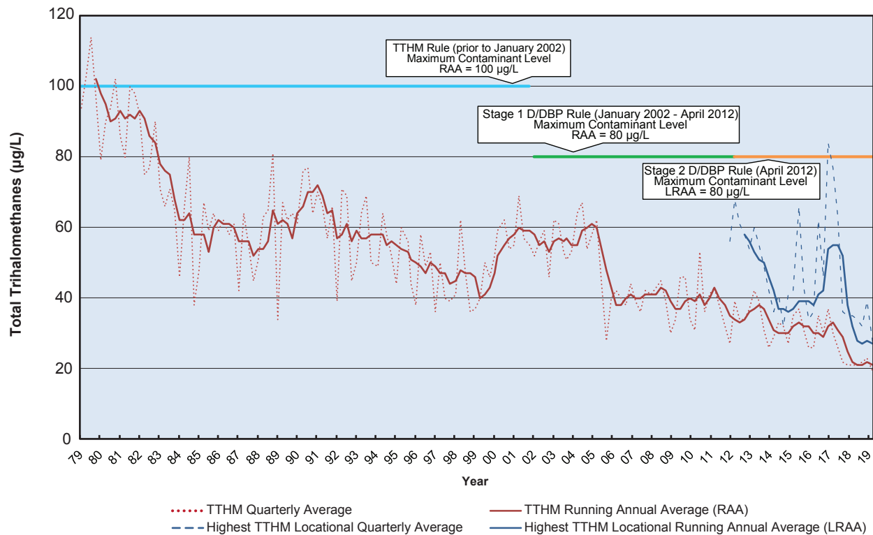
Figure 4-3. Total Trihalomethane (TTHM) Levels Throughout the Distribution System, Quarterly and Running Annual Averages 1979 to 2019
