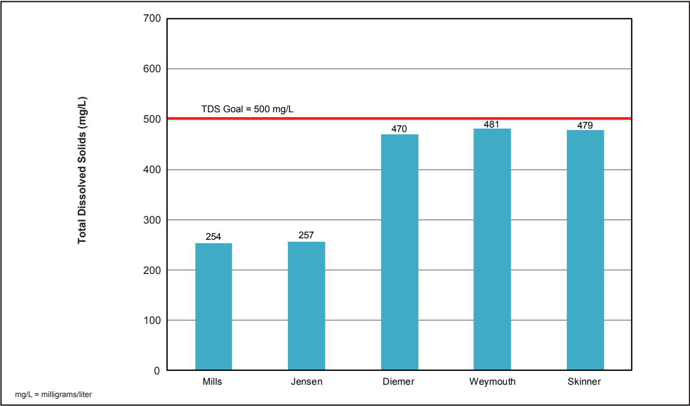
Figure 4-2. TDS (Total Dissolved Solids) in Plant Effluent, Annual Flow-Weighted Averages, FY 2018/19
