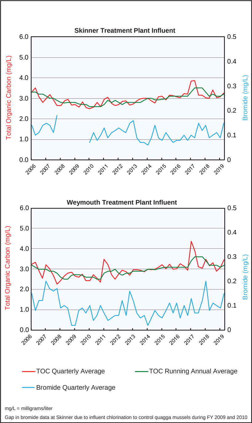
Figure 4-5 (continued). Total Organic Carbon (TOC) and Bromide Levels in Treatment Plant Influent, 2006 to 2019
