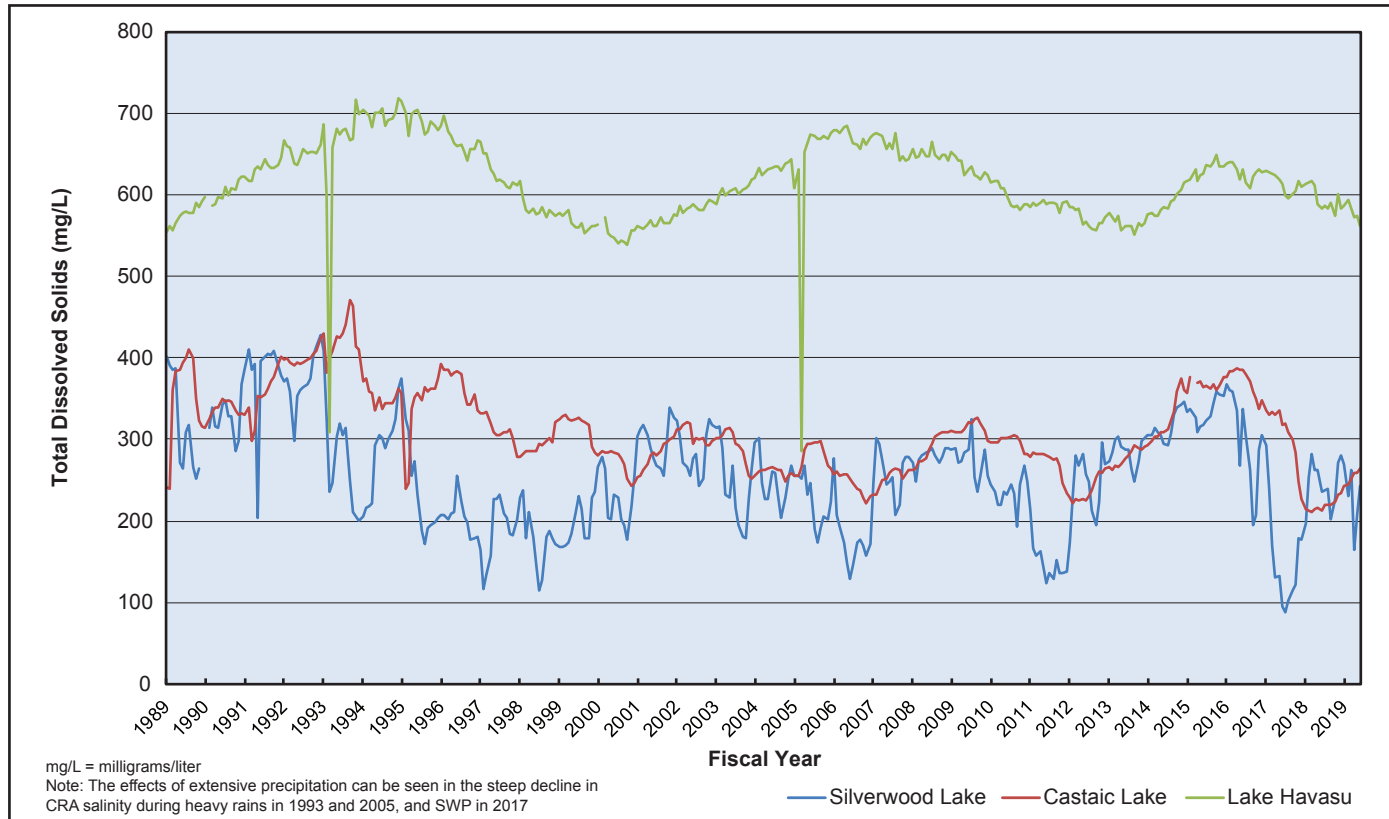
Figure 4-1. Total Dissolved Solids in East Branch State Water Project (Silverwood Lake), West Branch State Water Project (Castaic Lake), and Colorado River Aqueduct (Lake Havasu), 1989 to 2019
