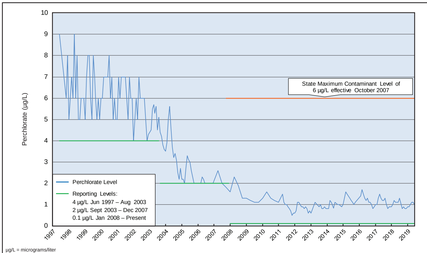
Figure 4-10. Perchlorate Levels at Lake Havasu, 1997 to 2019
