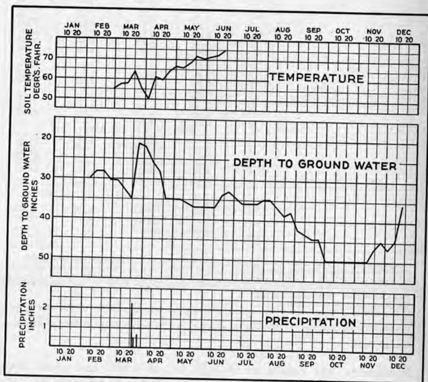
PLATE 21—Record of typical ground water well with contemporaneous precipitation and soil temperature, Richmond-Chase asparagus tract.
