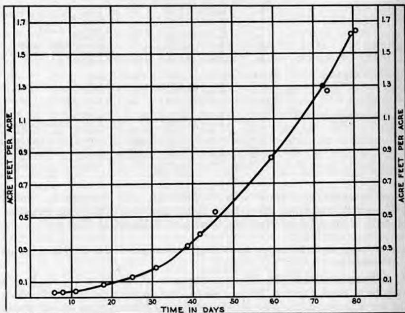
PLATE 24—Accumulated use of water by barley and weeds in Tank No. 22, Medford Island, 1925.
