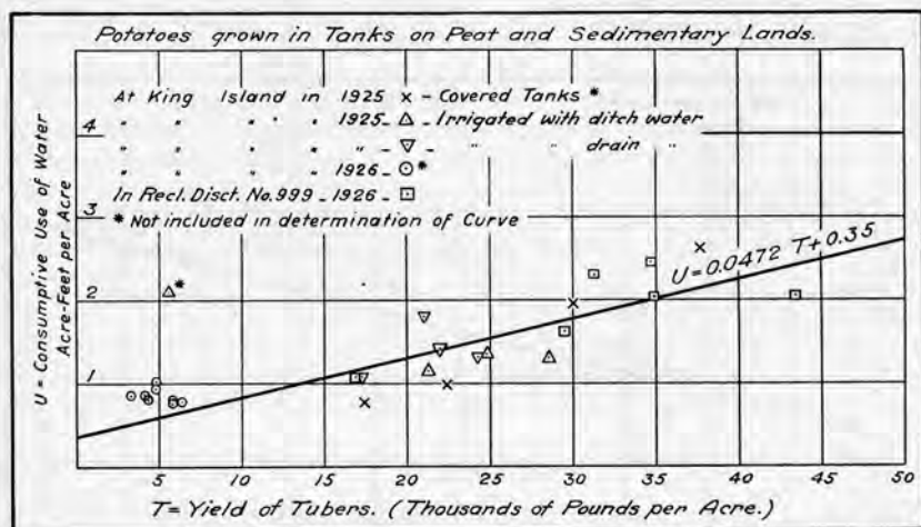
PLATE 14—Relation of consumptive use of water to yield for potatoes grown in tanks on peat and sedimentary lands.
