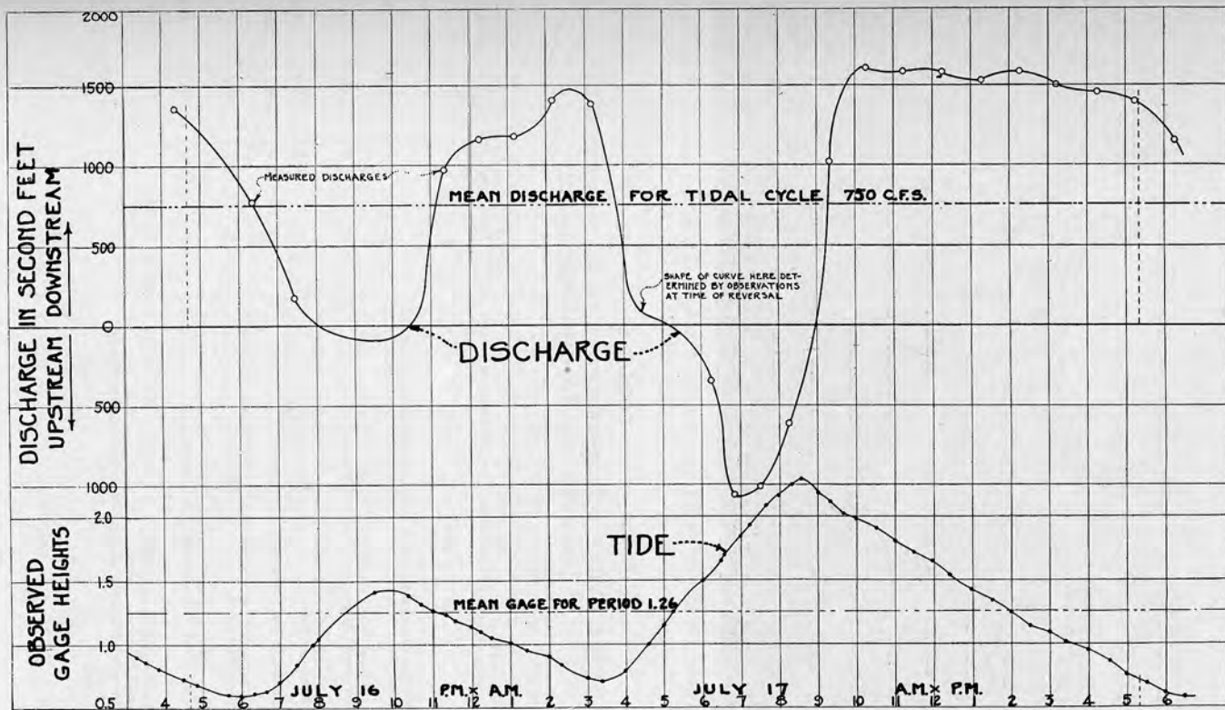
PLATE 1—Relation between Tide and Discharge of the Sacramento River near Sacramento as shown by Tidal Cycle Measurement, July 16-17, 1924.
