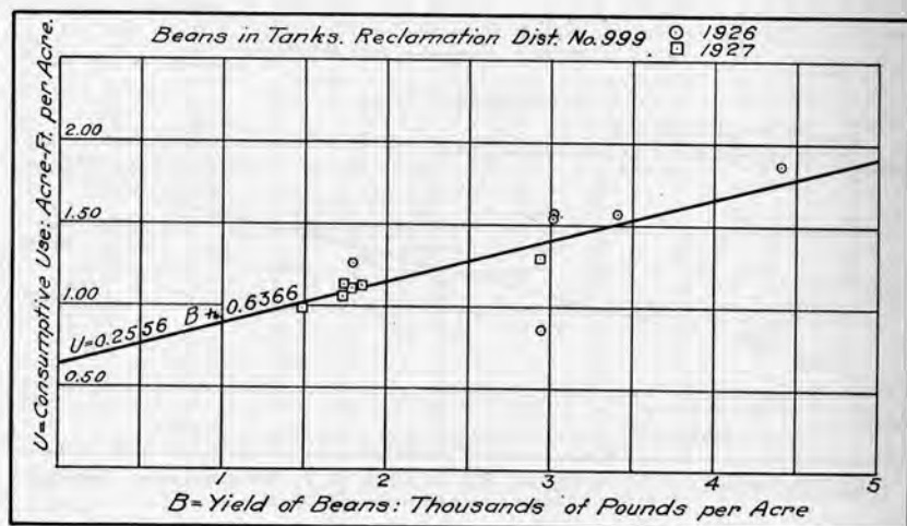
PLATE 15—Relation of consumptive use of water to yield for beans grown in tanks.
