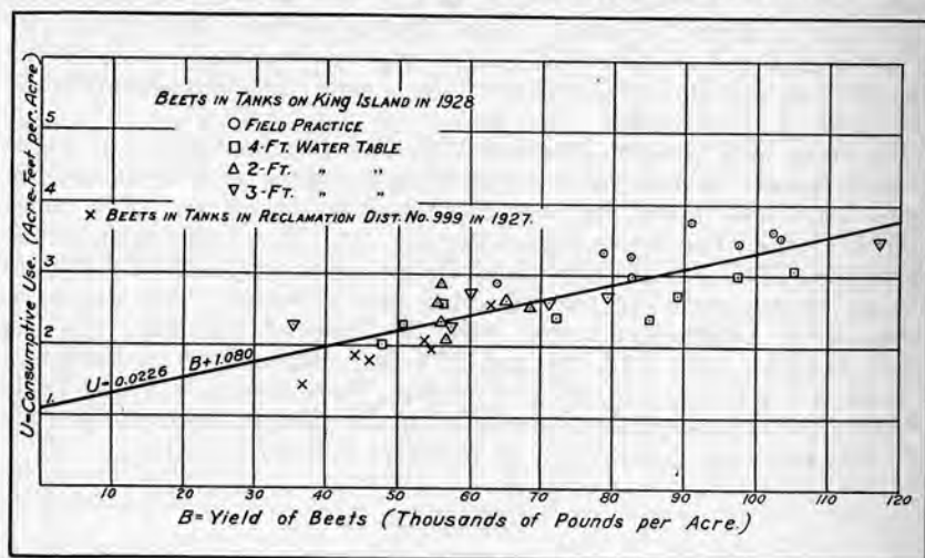
PLATE 16—Relation of consumptive use of water to yield for beets grown in tanks.
