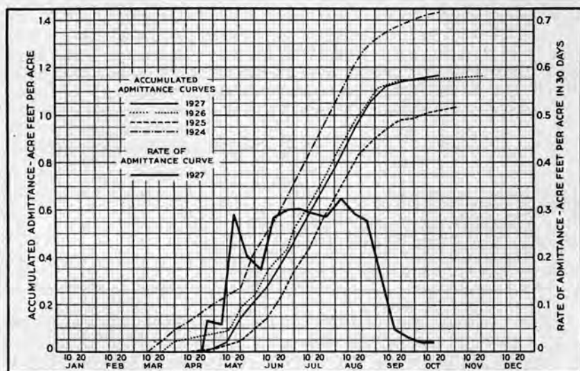
PLATE 26—Accumulated admittance of water, 1924 to 1927, inclusive, and rates of admittance, 1927, for pumping plants, siphons and gravity inlets. Lower unit, Reclamation District No. 999.
