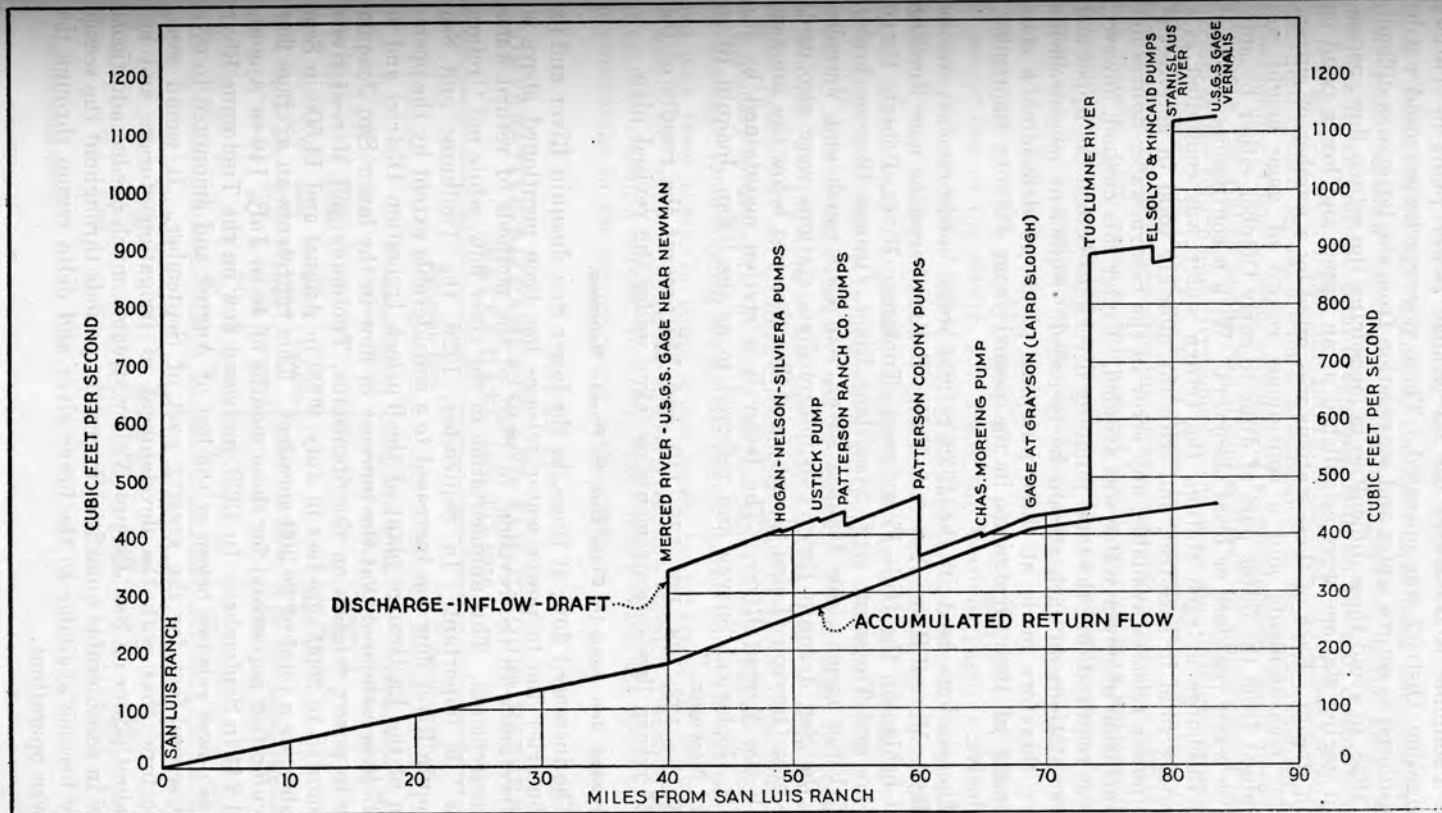
PLATE 6—San Joaquin River Return Flow, San Luis Ranch to Vernalis, July 1 to September 30, 1928
