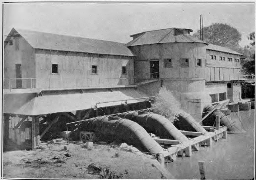
FIG. 2. Pumping plant of Glenn-Colusa Irrigation District for diverting water from Sacramento River into Central Canal.
