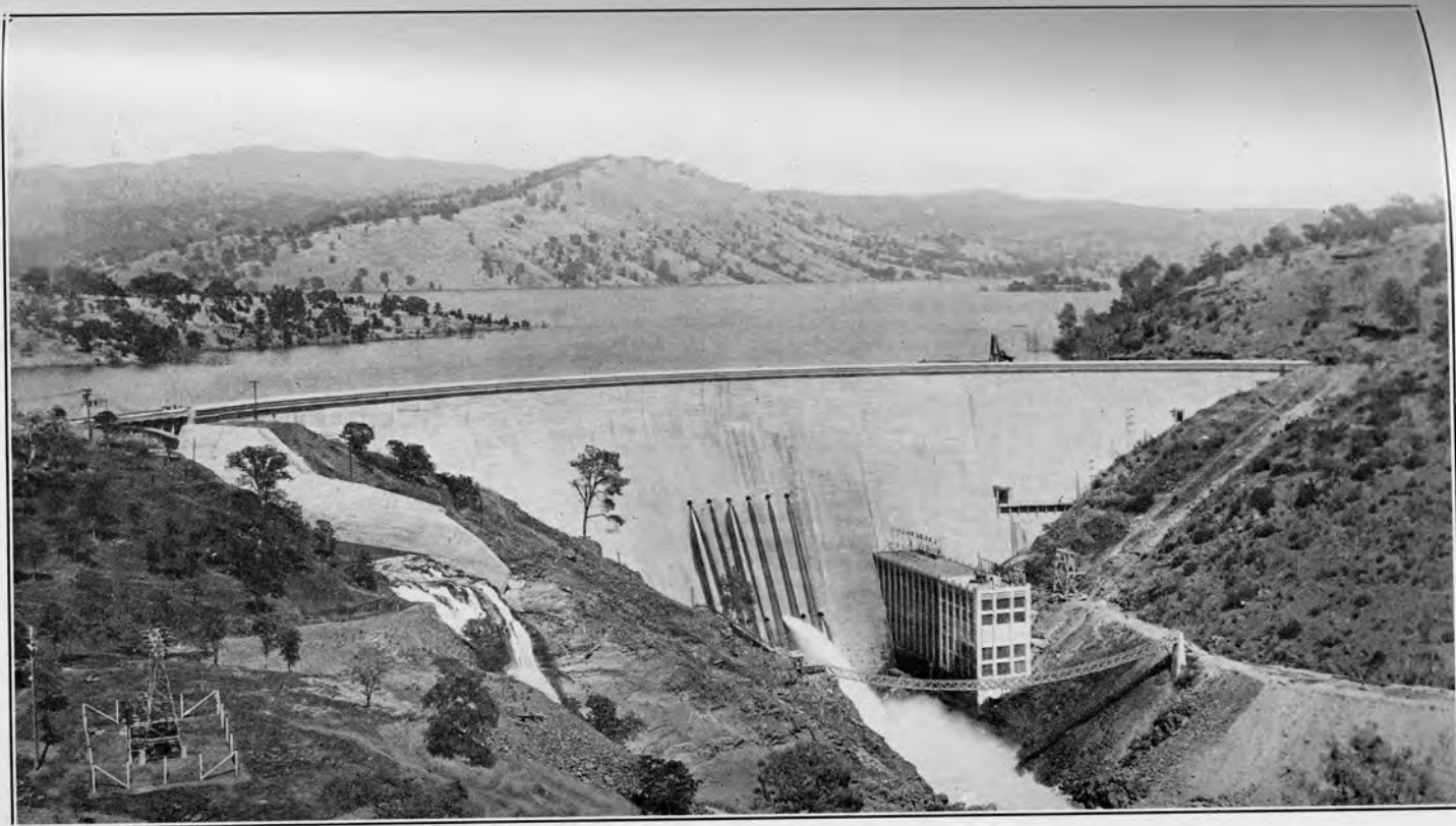
Don Pedro Dam, Reservoir, and Power House, Turlock and Modesto irrigation districts.
