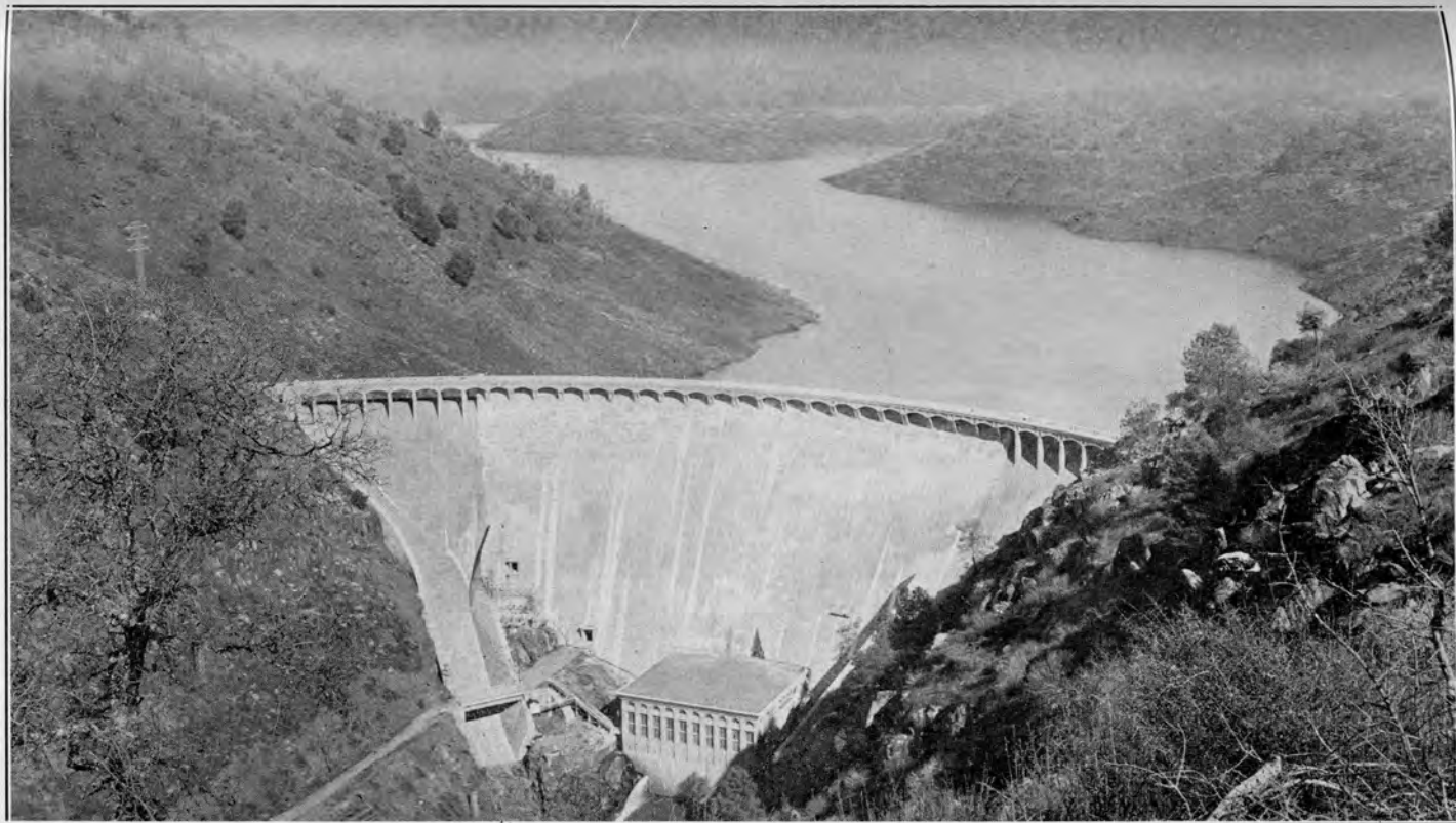
Exchequer Dam and Power House and Lake McClure at low water stage, Merced Irrigation District.
