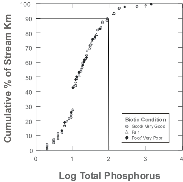
Figure 5. Cumulative distribution function of total phosphorous concentration for 80 target-sampled sites in central & southern coastal California; 10% of stream km are impaired at phosphorous threshold of 100 ppb (log = 2).
