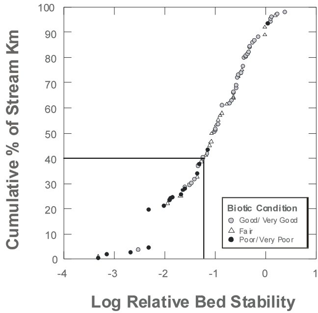
Figure 3. Cumulative distribution function of relative bed stability for 80 target-sampled sites in central & southern coastal California; 40% of stream km are impaired at LRBS threshold of -1.25.
