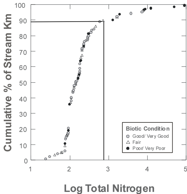
Figure 4. Cumulative distribution function of total nitrogen concentration for 80 target-sampled sites in central & southern coastal California; 11% of stream km are impaired at nitrogen threshold of 750 ppb (log = 2.87).
