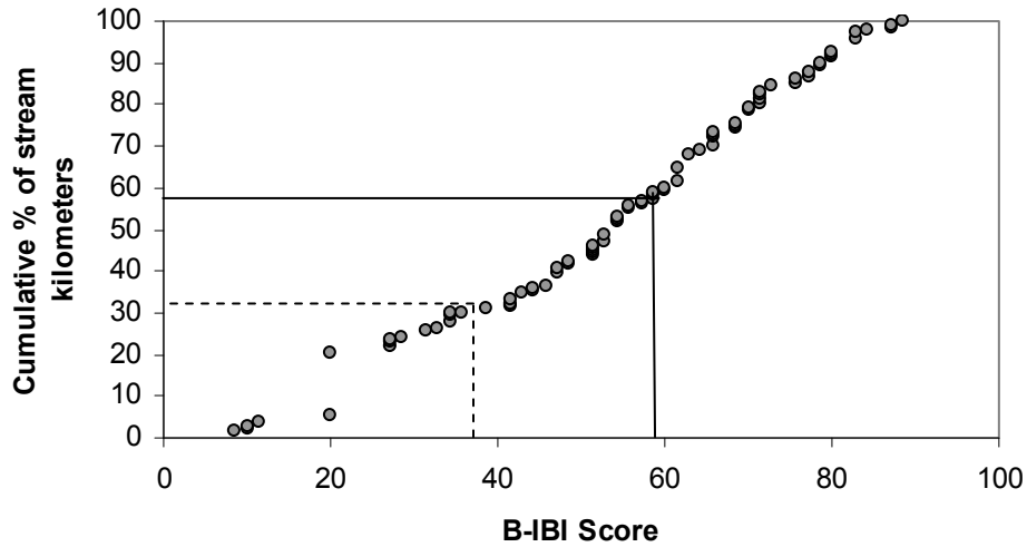
Figure 2. Cumulative distribution function of B-IBI scores for 80 target-sampled sites in central & southern coastal California showing two potential B-IBI impairment thresholds: --- B-IBI =37 (“Poor”); — B-IBI = 59 (“Fair”).
