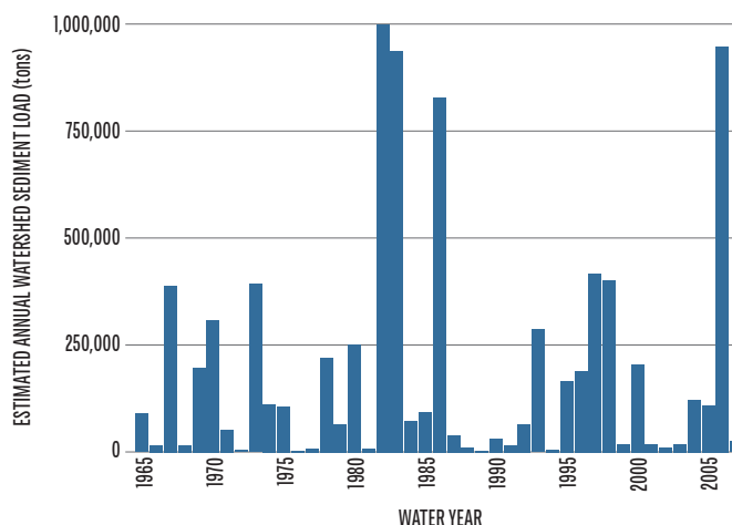
Walnut Creek watershed total sediment load (1965-2007).
