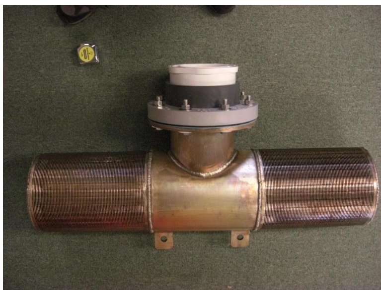
Figure 2. Wedgewire screen module used in testing during studies for Santa Cruz and Soquel Creek Water Districts in 2009 and 2010. The screen had a slot width of 2 mm (0.8 in) and was sized to ensure a maximum through screen velocity of 0.1 mps (0.33 fps).
