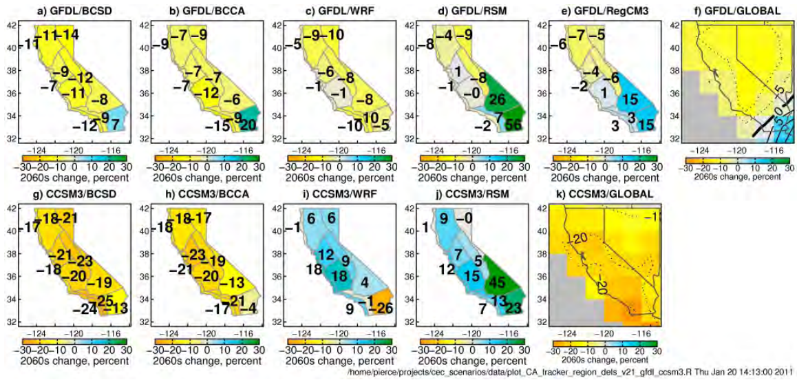
Figure 9: Yearly Precipitation Change (% 2060–2069 Compared to 1985–1994) from Each Downscaling Technique Applied to the GFDL 2.1 (top row) and CCSM3 (bottom row) Global Models. The yearly precipitation changes from the global models are shown in panels f and k, for comparison.
