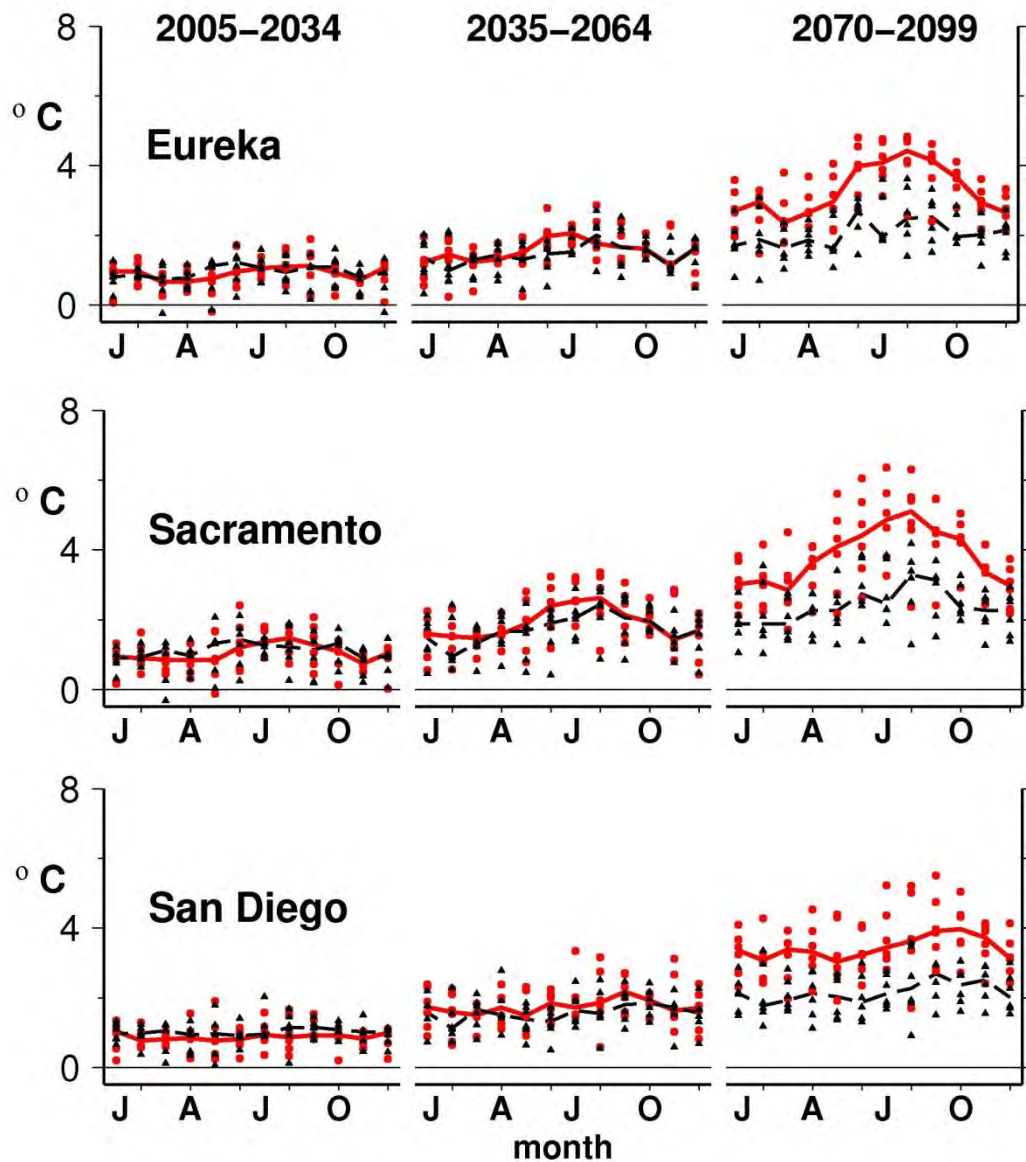
Figure 4: Monthly BCSD Simulated Temperature Changes ( ^{\circ}\text{C} ) for Eureka, Sacramento, and San Diego for Six GCMs. Changes (from 1961–1990) are shown for three time periods: early century (2005–2034; left), mid-century (2035–2064; middle) and late century (2070–2099; right). Changes are shown in each panel for January (left) to December (right). Black and red symbols show changes for B1 and A2 emission scenarios, respectively. Black (dashed; B1) and red (solid; A2) lines show the median value for the six GCMs, which are those listed in Figure 2.
