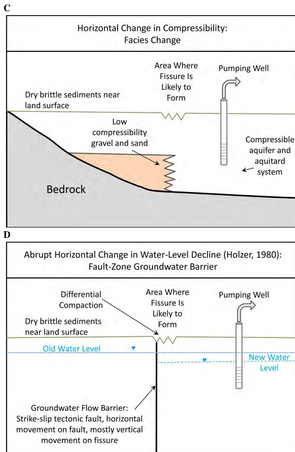
Figure 3-4 A-D. Schematic of differential compaction settings for earth fissures. A) Wells pumping near a substantial change in the thickness of compressible aquifer materials at a basin-bounding fault trigger fissuring. B) High total compaction in thick sediments triggers fissuring where sediments are thin over a buried bedrock high. C) Fissure forms where less compressible sand and gravel transition to highly compressible clay and silt. D) Sediments are uniformly compressible, but a fissure forms where a fault barrier prevents groundwater from flowing toward pumping wells.
